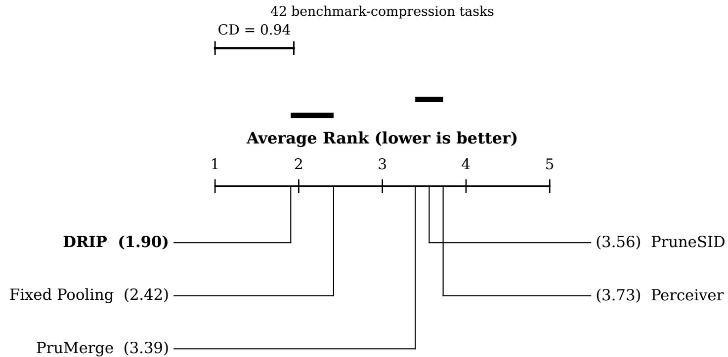
(a) Overall
