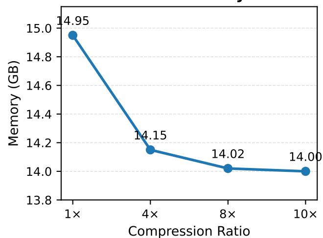
GPU Memory
