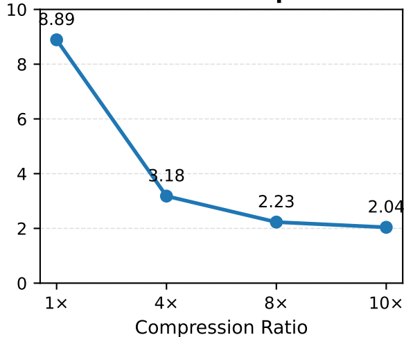
Forward Compute
