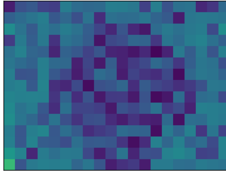
pancake: 15×20
