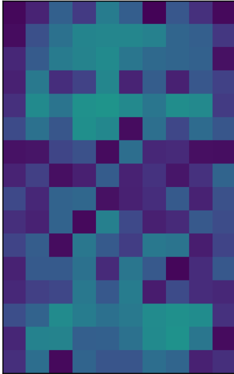
text_dreams: 16×10
