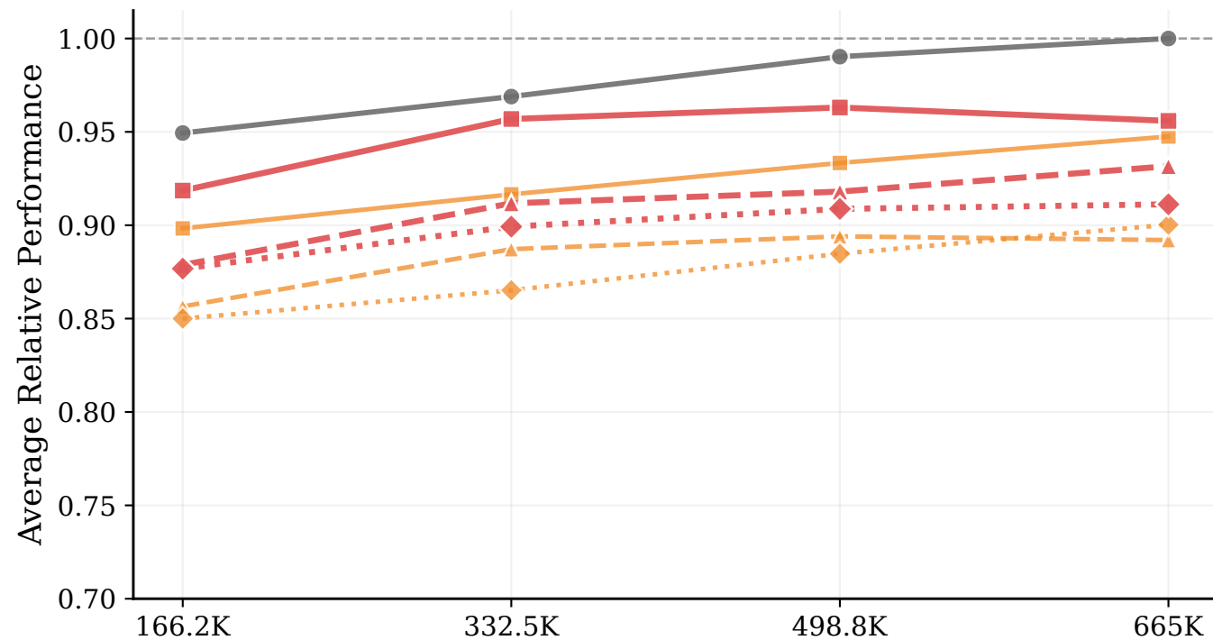
Overall Performance
