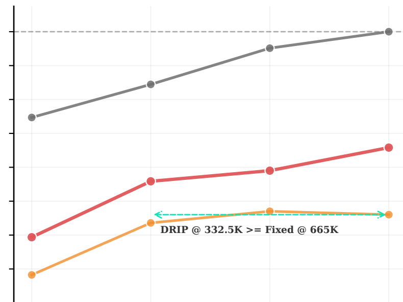
8x Compression
