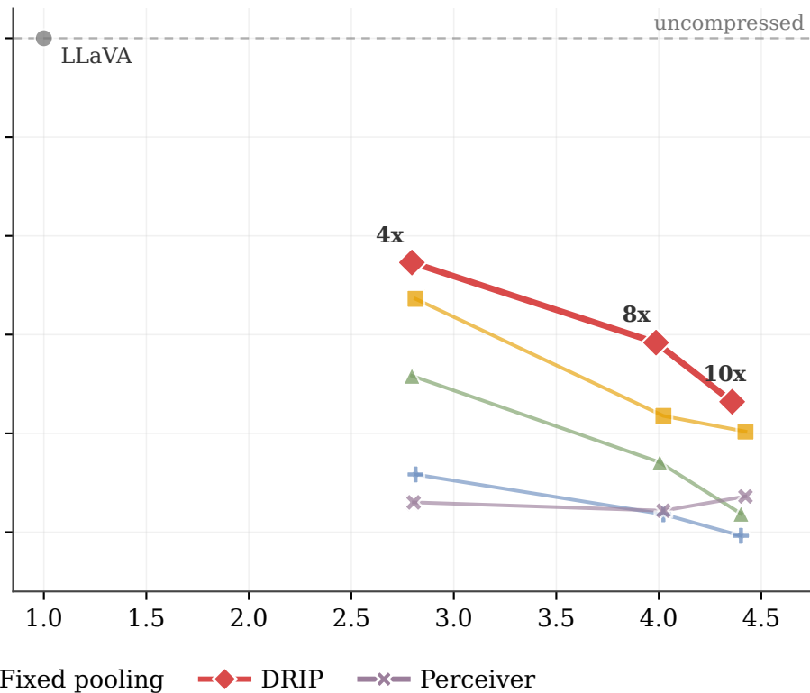
OCR Performance
