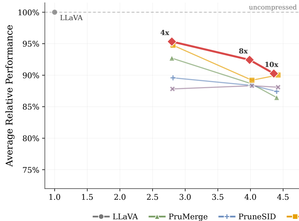
Overall Performance
