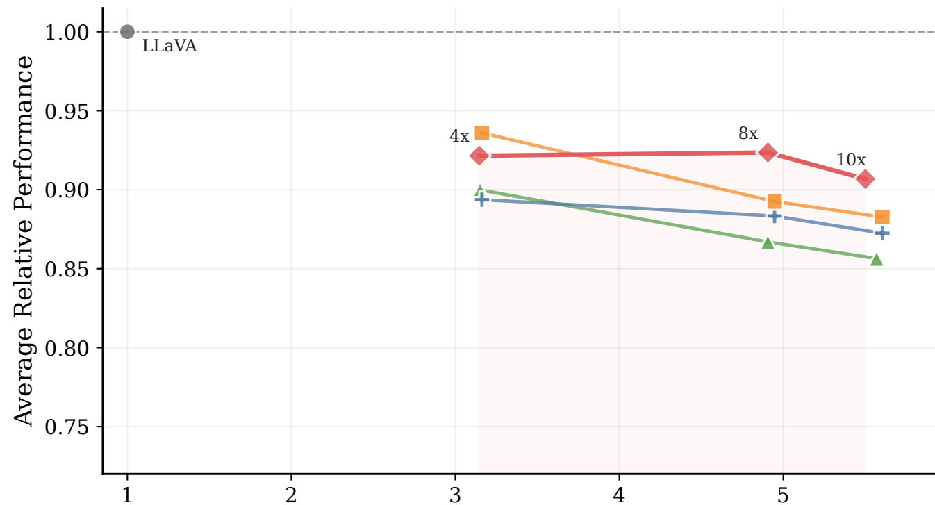
Overall Performance
