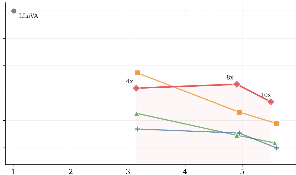
OCR Performance
