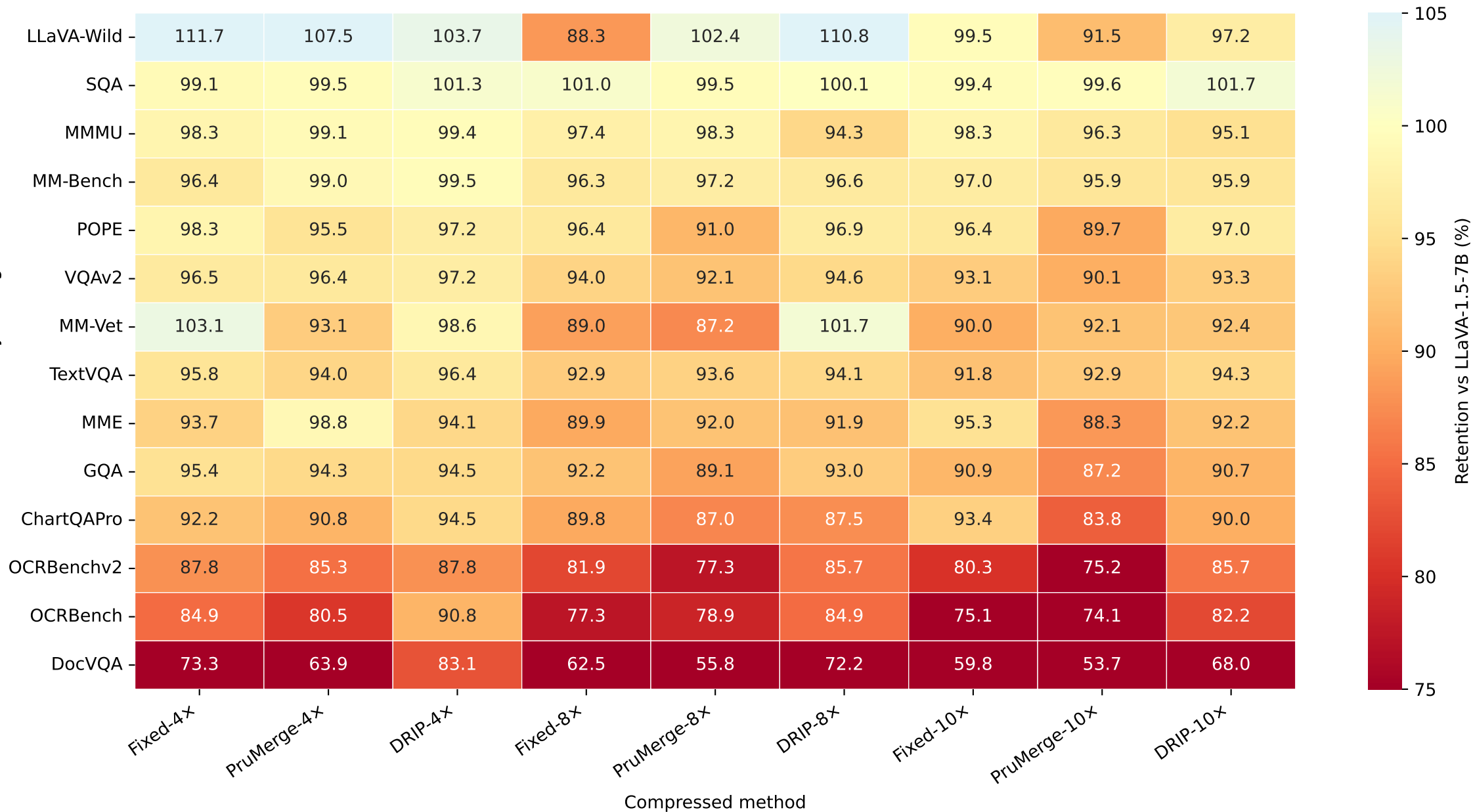
Benchmark Compressibility Heatmap
