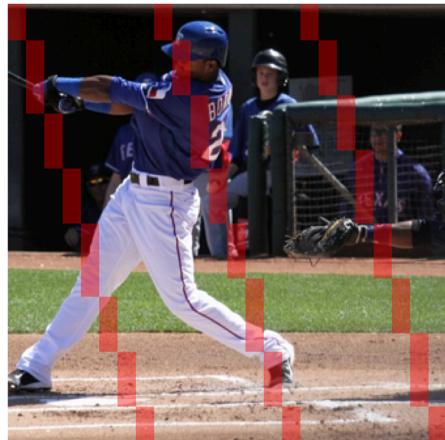
Fixed Pooling: "17"
