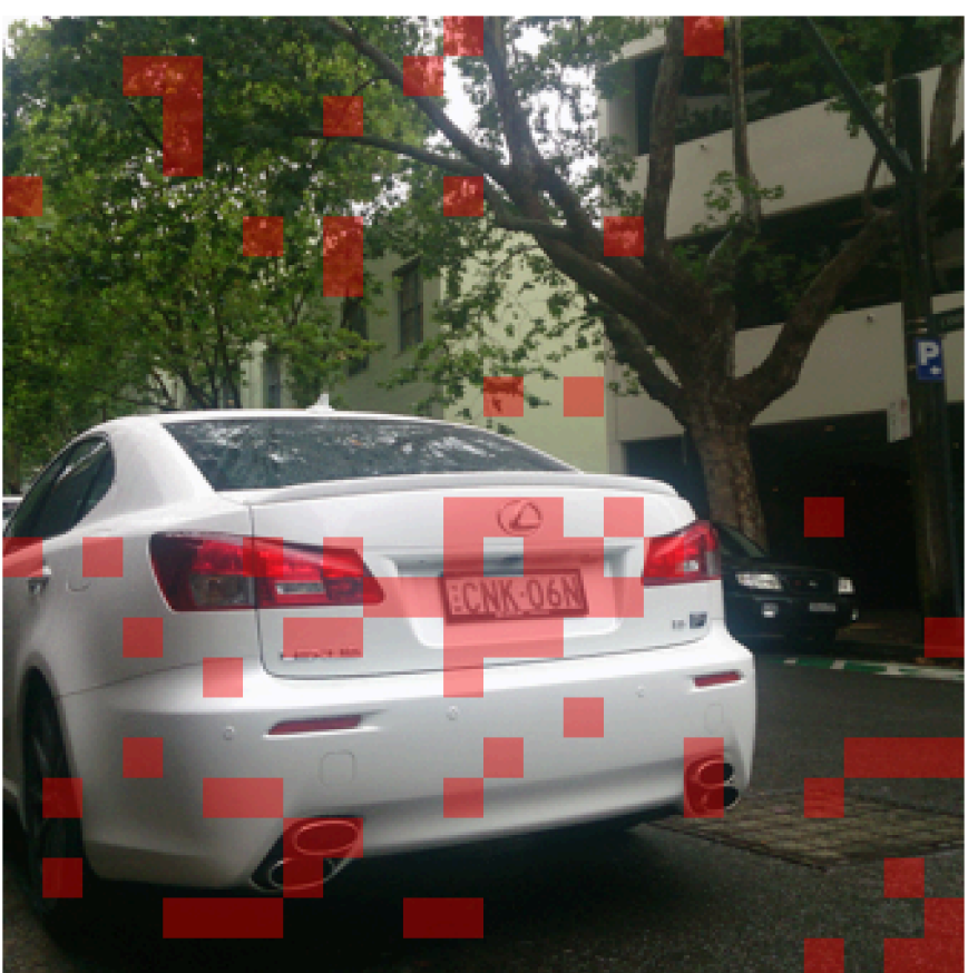
DRIP: "Lexus"
