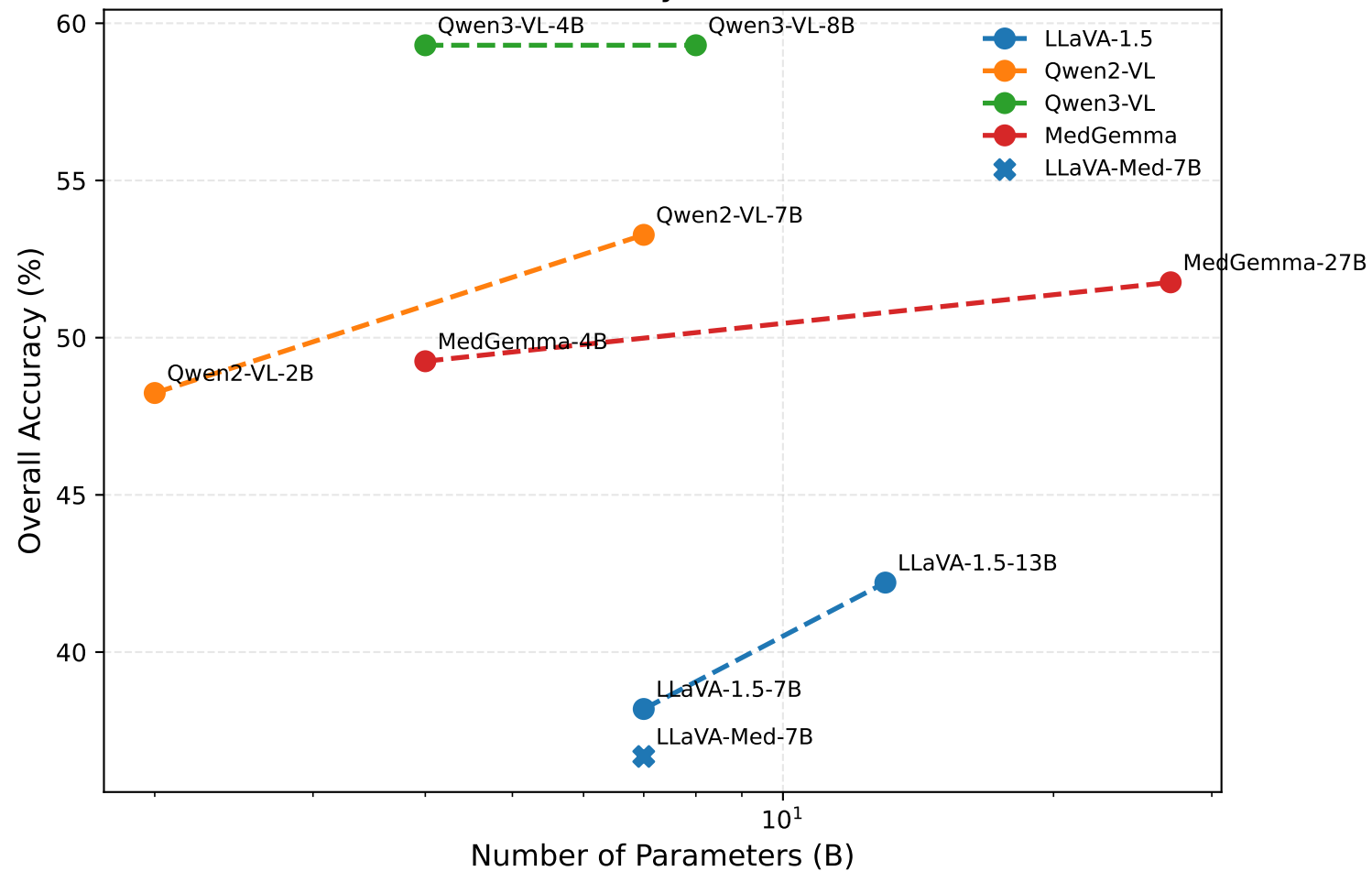
Overall Accuracy vs. Model Size
