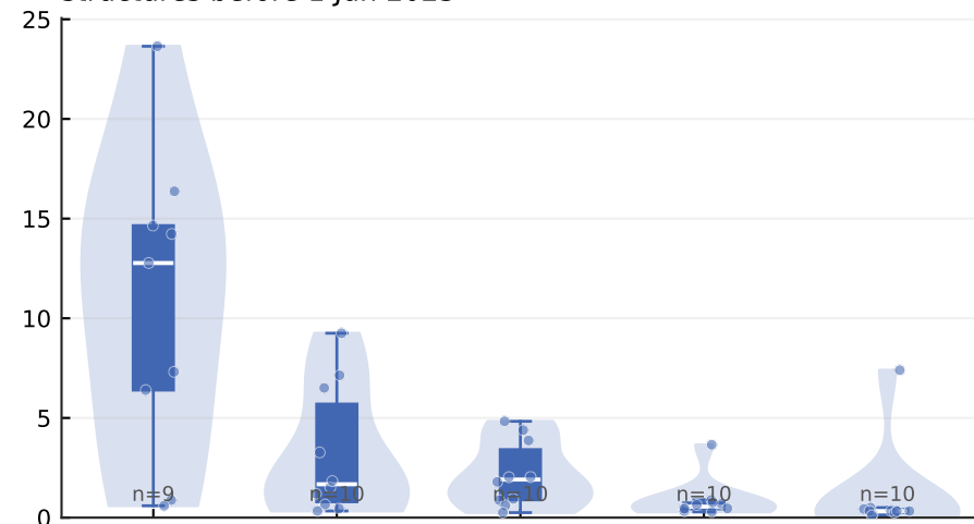
Boltz-2 structures before 1 Jun 2023
