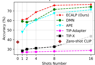
Accuracy on EuroSAT
