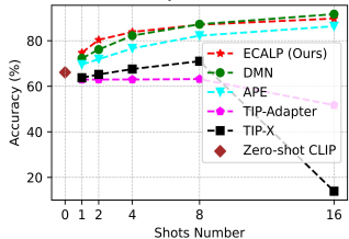
Accuracy on UCF101
