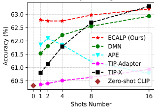
Accuracy on StanfordCars
