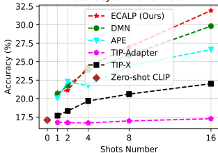
Accuracy on FGVCaircraft
