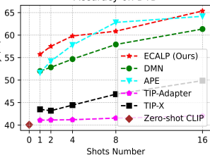
Accuracy on SUN397
