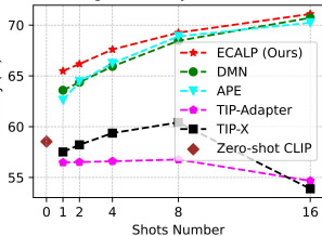
Accuracy on DTD
