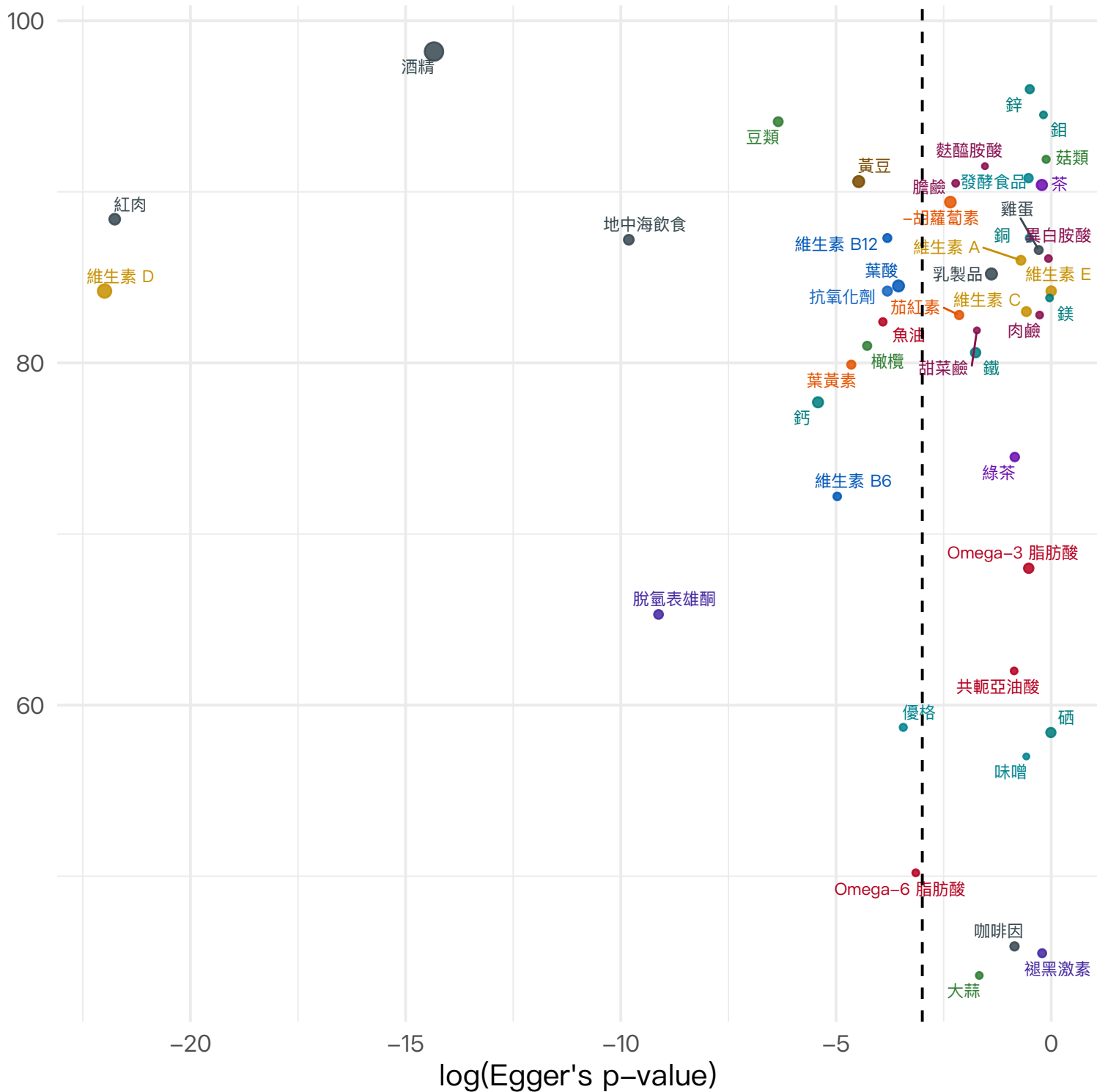
Egger's Test log(p-value) vs Heterogeneity – Breast cancer
