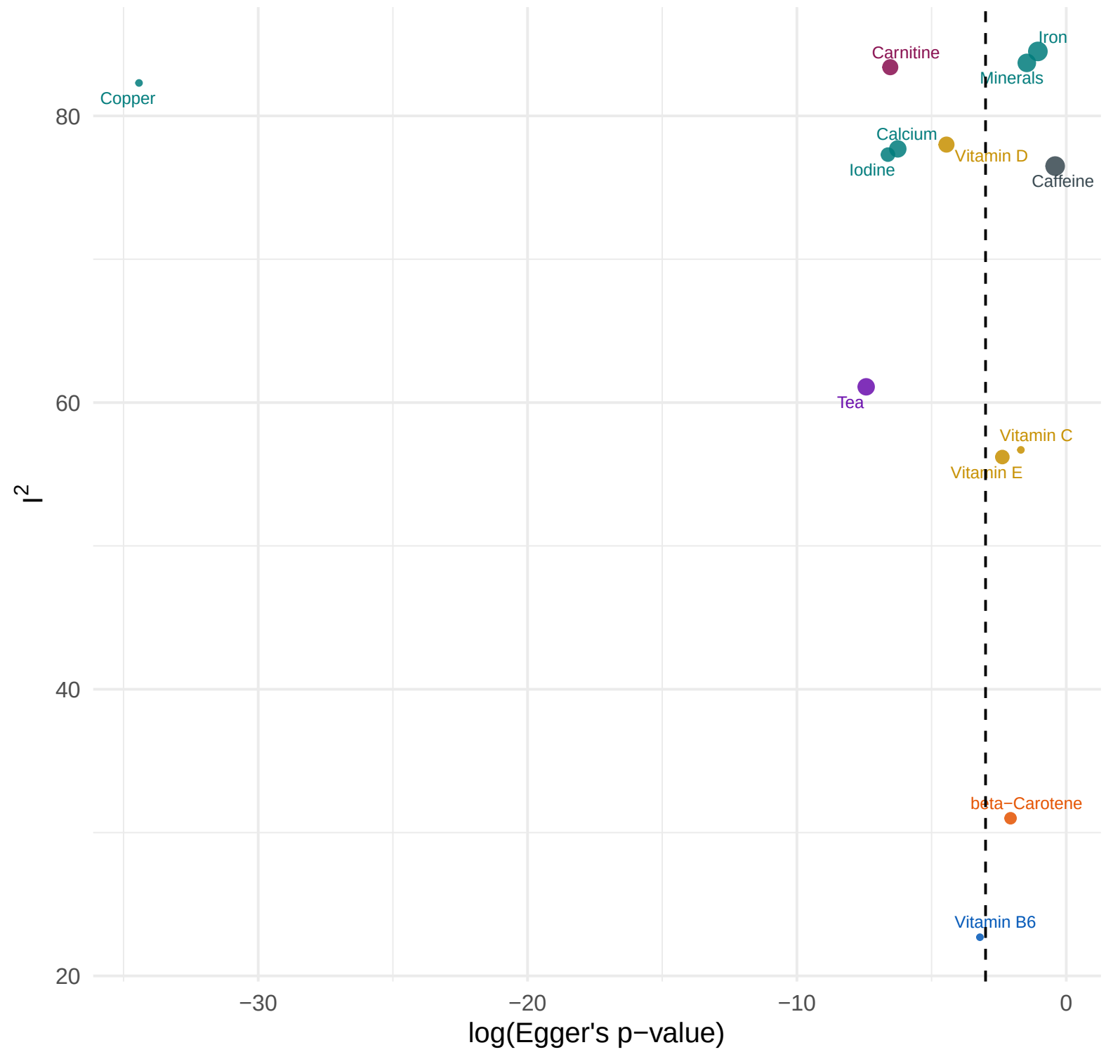
Egger's Test log(p-value) vs Heterogeneity
