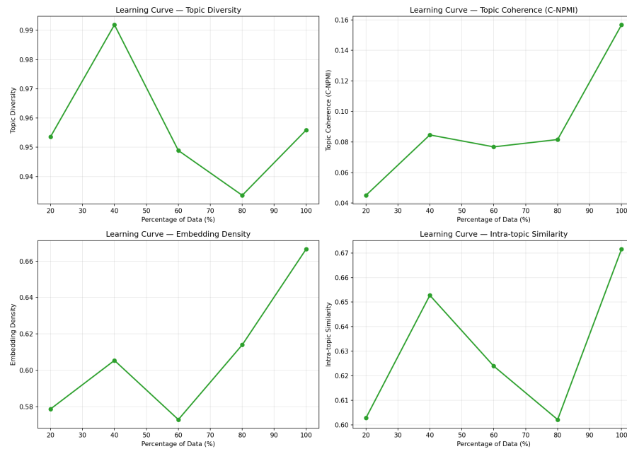
Gambar 4.2: Kurva Pembelajaran (Learning Curve) Model Usulan (Proposed)
