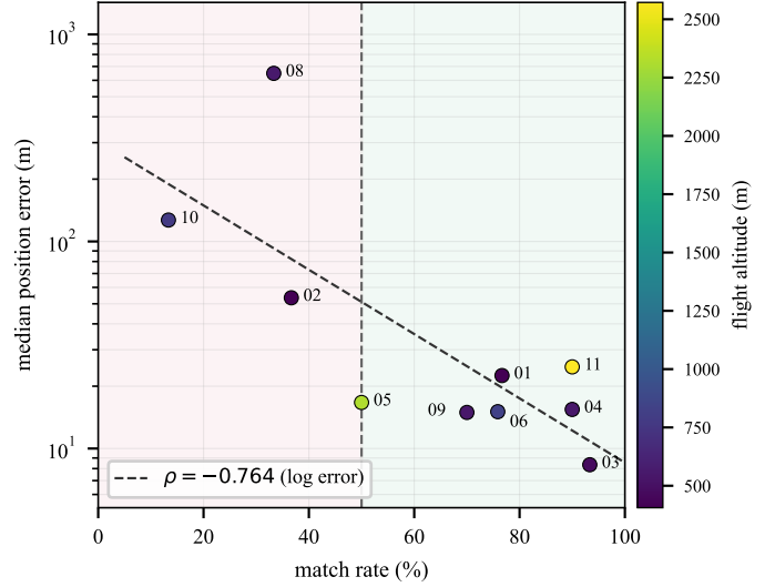
Fig. 3. Match rate against final accuracy across the ten flights. Match rate is measured with the true position given, so it describes the data rather than the algorithm, and it can be evaluated on a planned route before flying. Colour encodes altitude, which does not separate the groups: the 2572 m flight (11) succeeds and the 551 m flight (08) fails.
