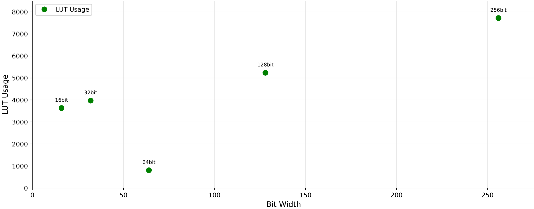
LUT Usage vs Bit Width for Comba Multiplication (Linear Scale)
