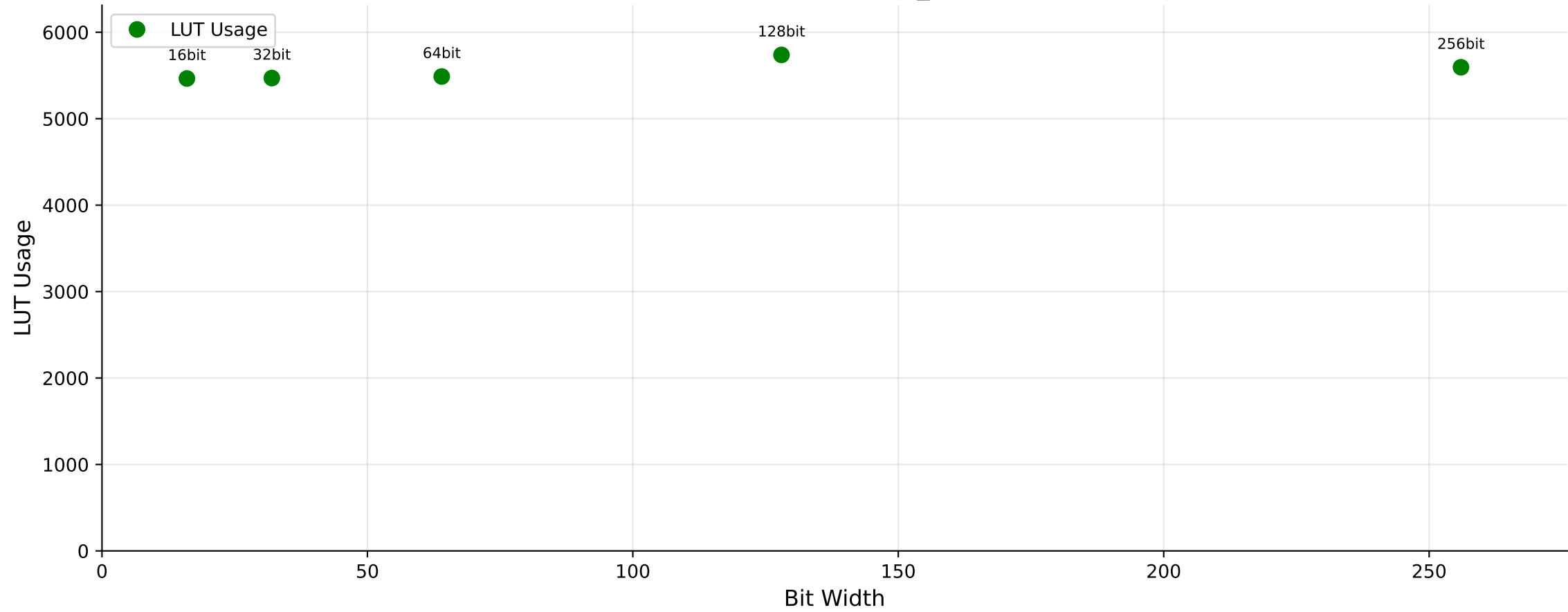
LUT Usage vs Bit Width for mul_ver2 (Linear Scale)
