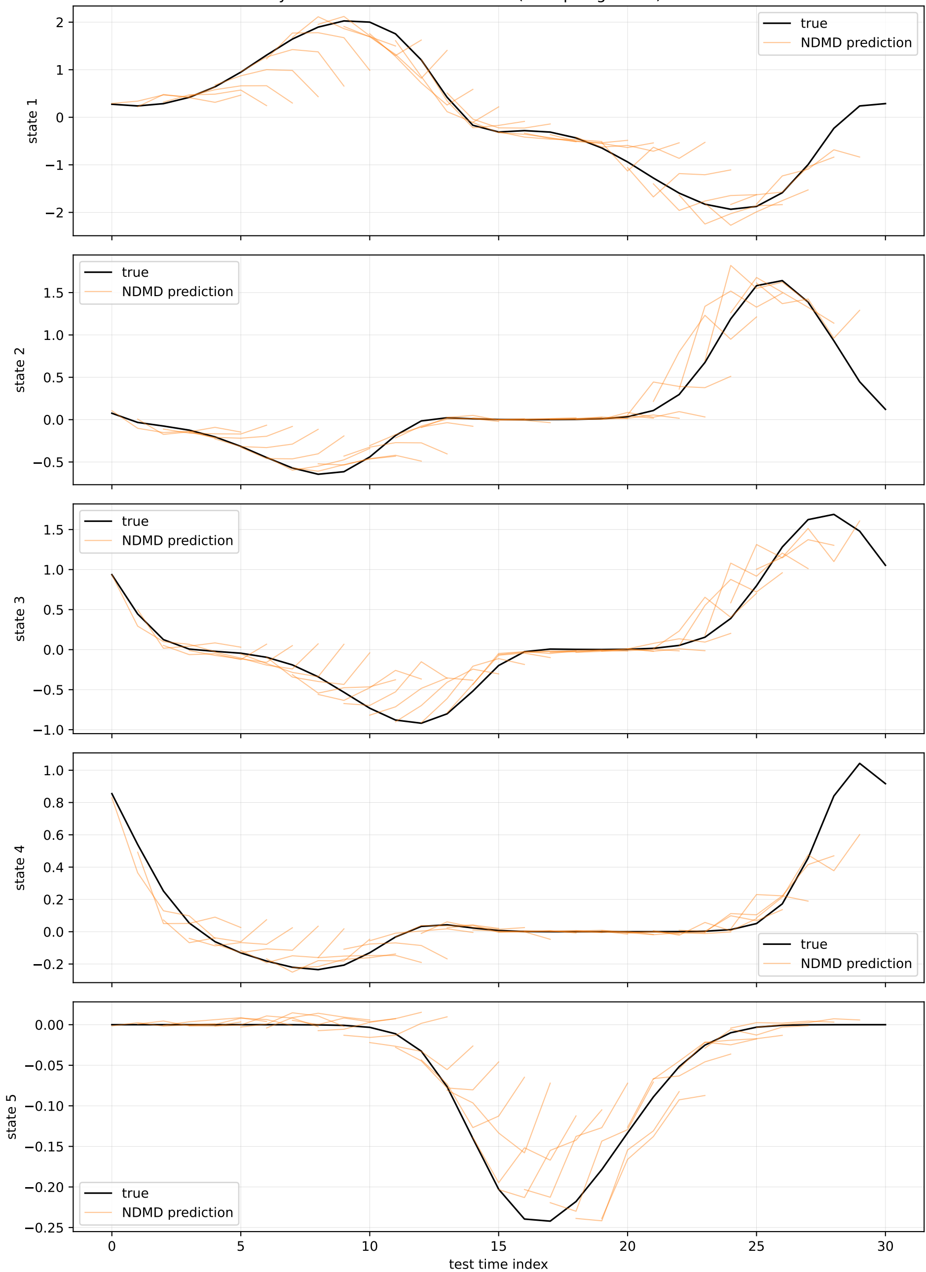
Cylinder Flow NDMD Prediction (5-step segments)
