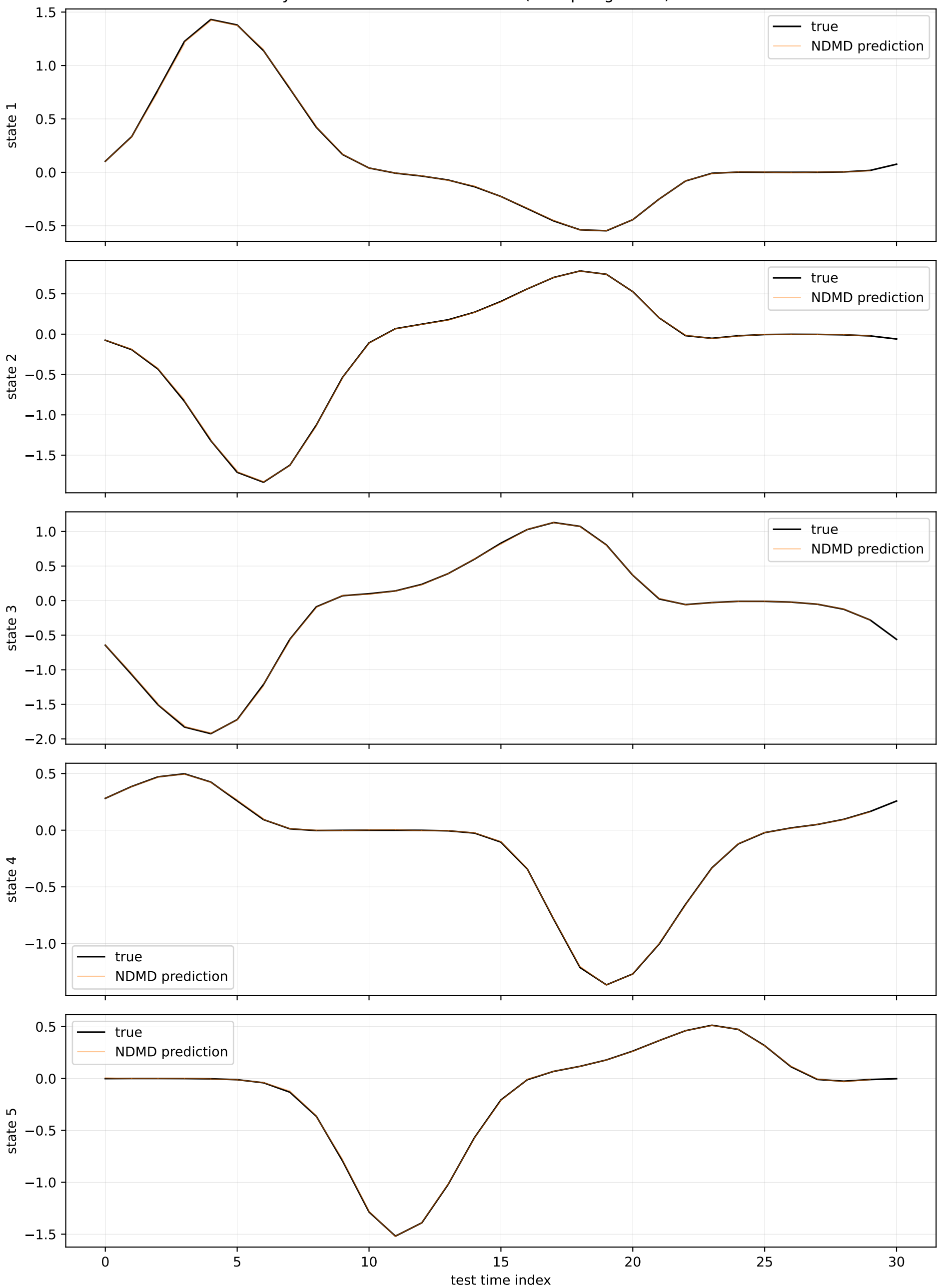
Cylinder Flow NDMD Prediction (2-step segments)
