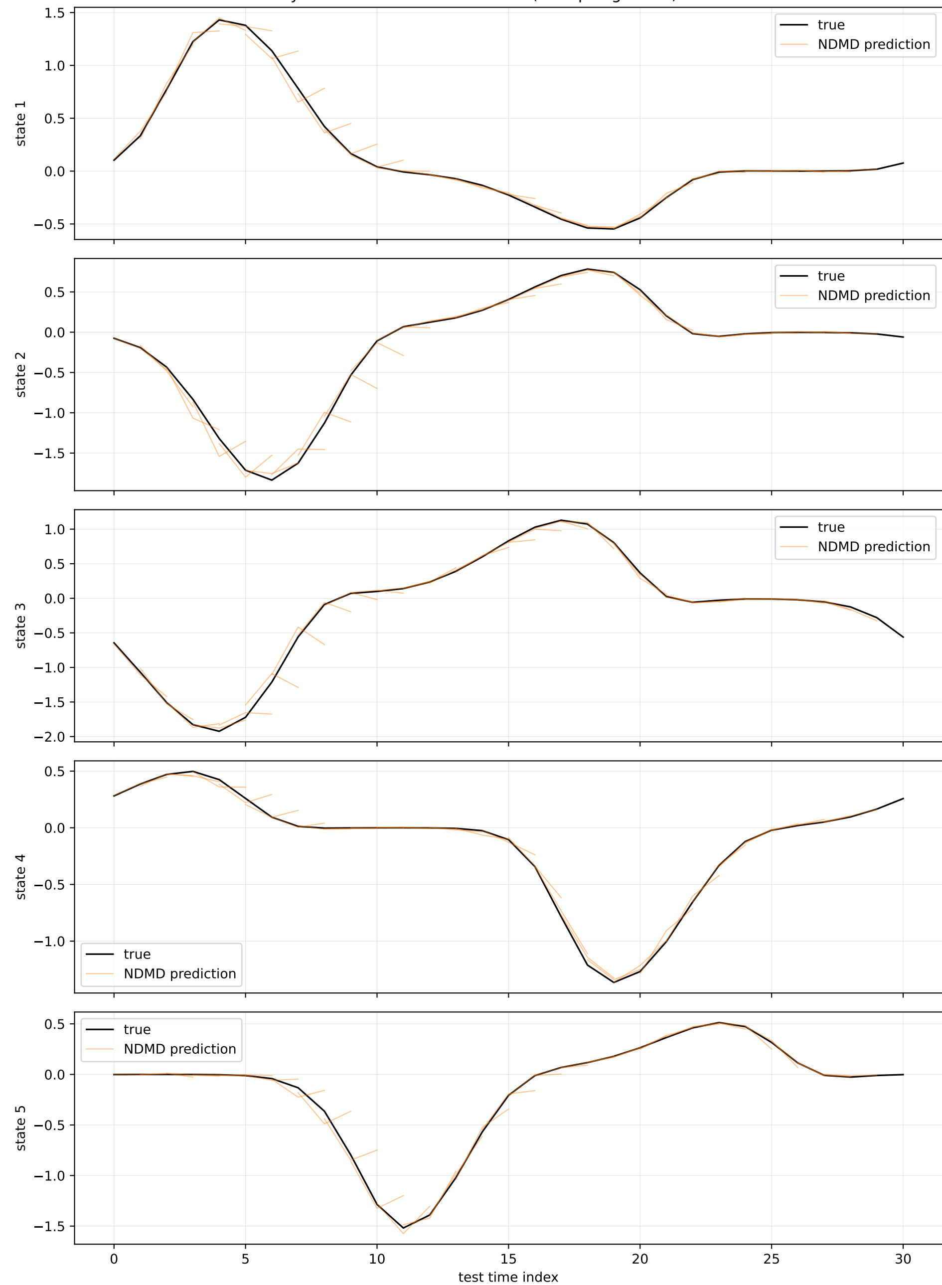
Cylinder Flow NDMD Prediction (3-step segments)
