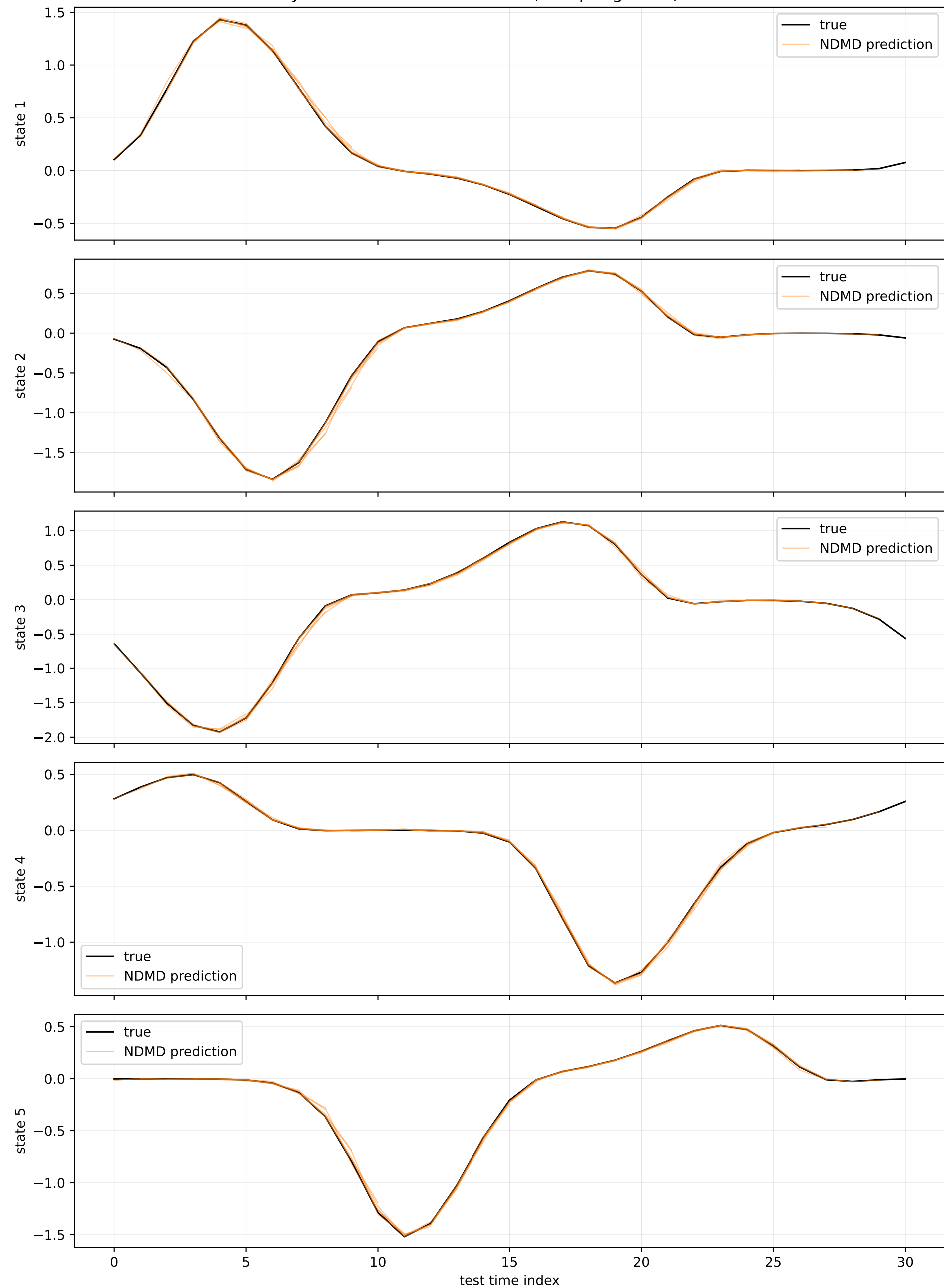
Cylinder Flow NDMD Prediction (6-step segments)
