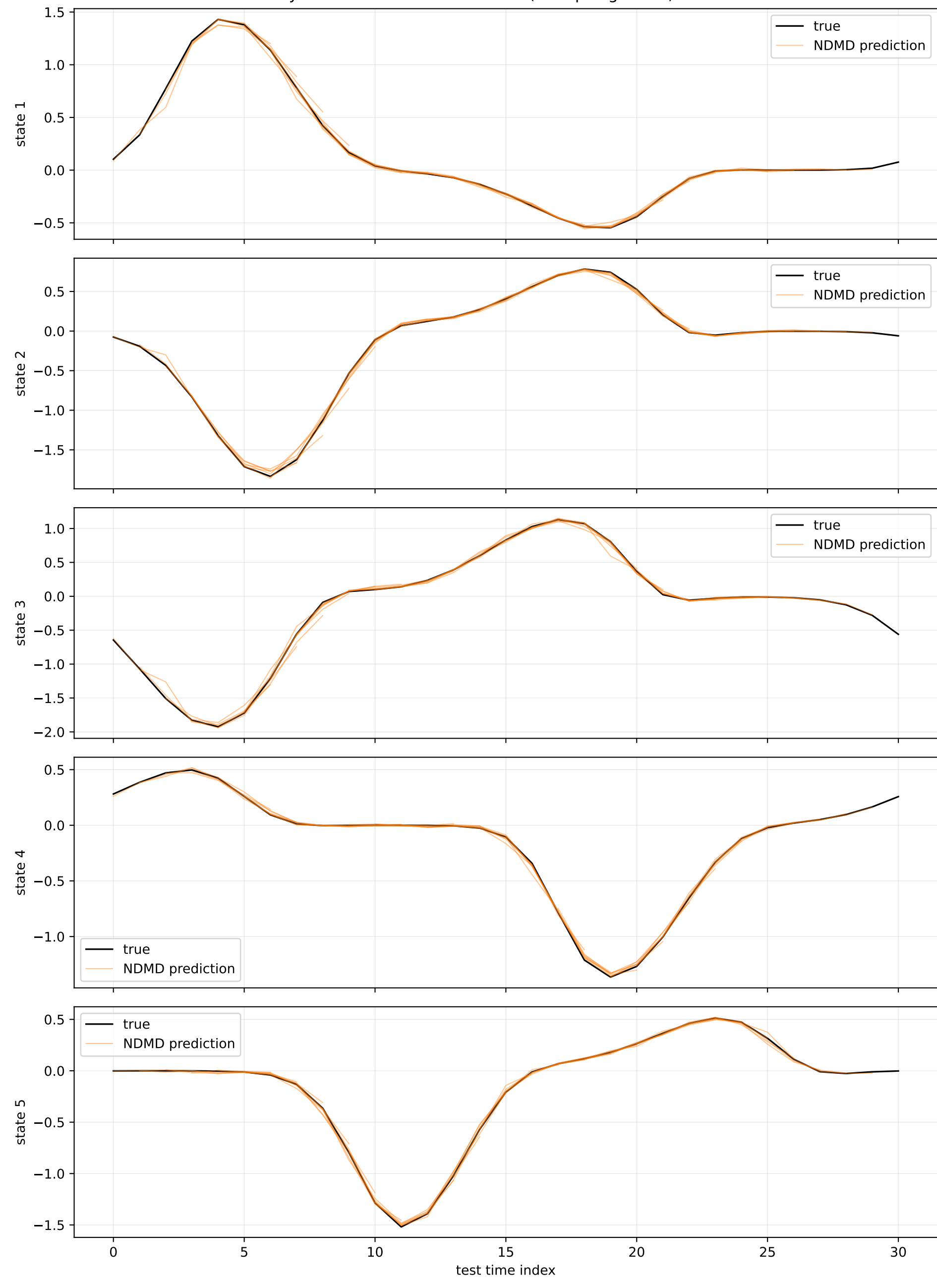
Cylinder Flow NDMD Prediction (7-step segments)
