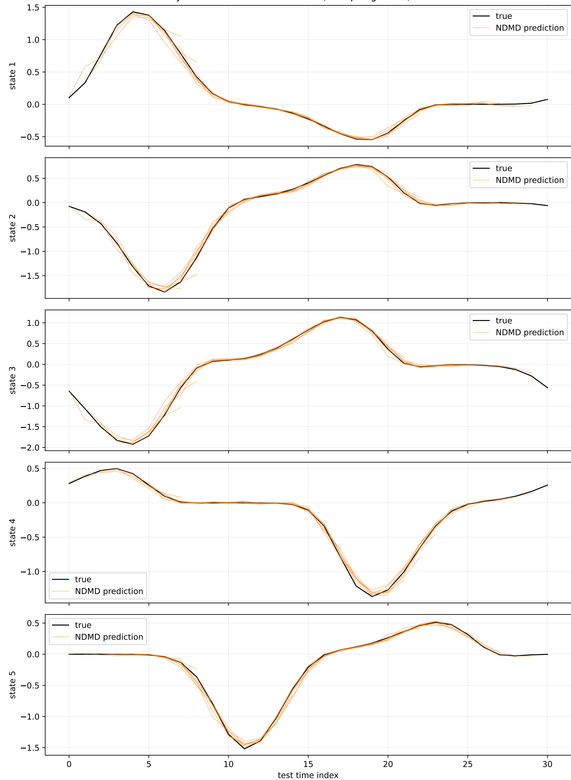
Cylinder Flow NDMD Prediction (8-step segments)
