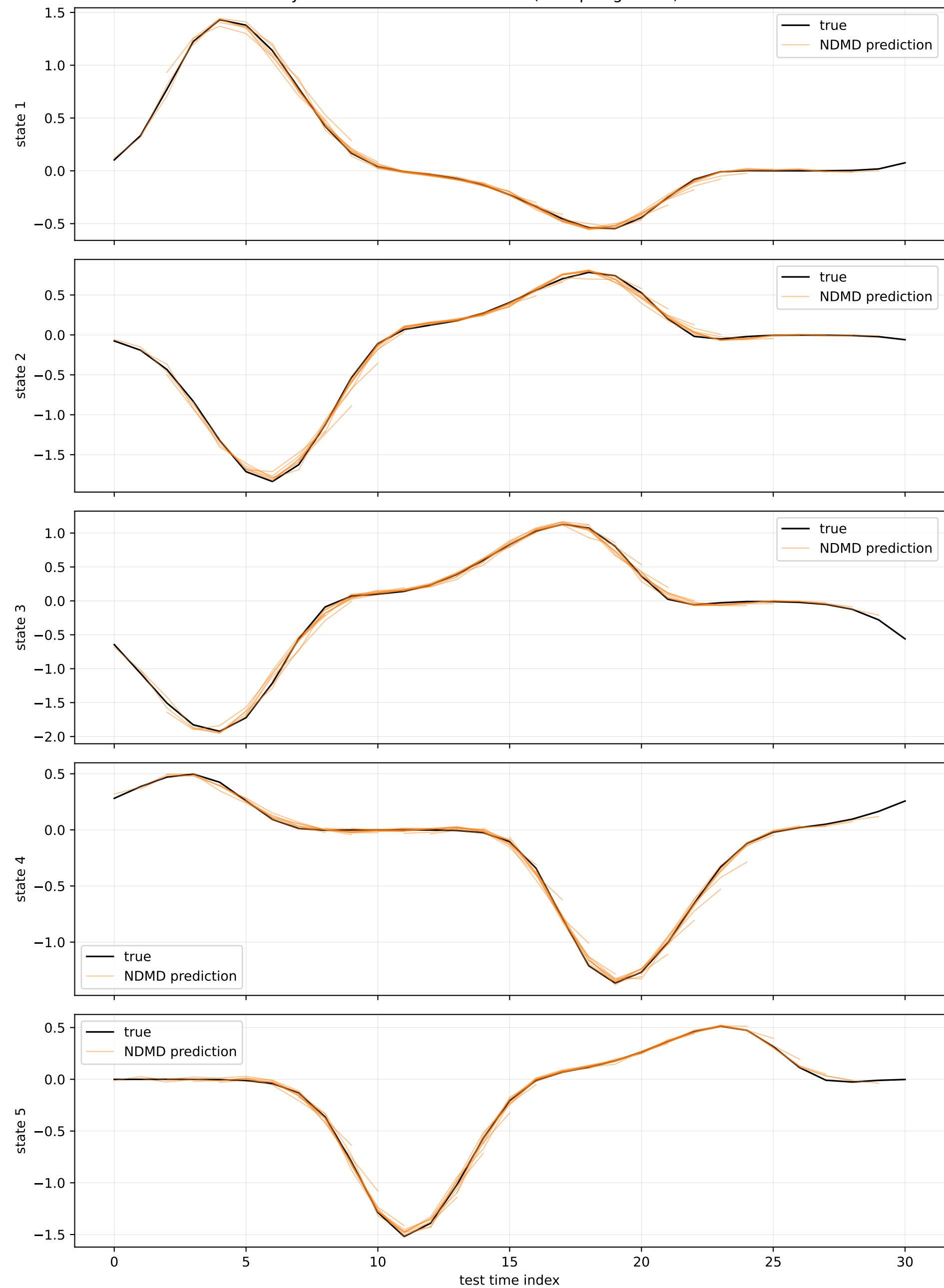
Cylinder Flow NDMD Prediction (9-step segments)
