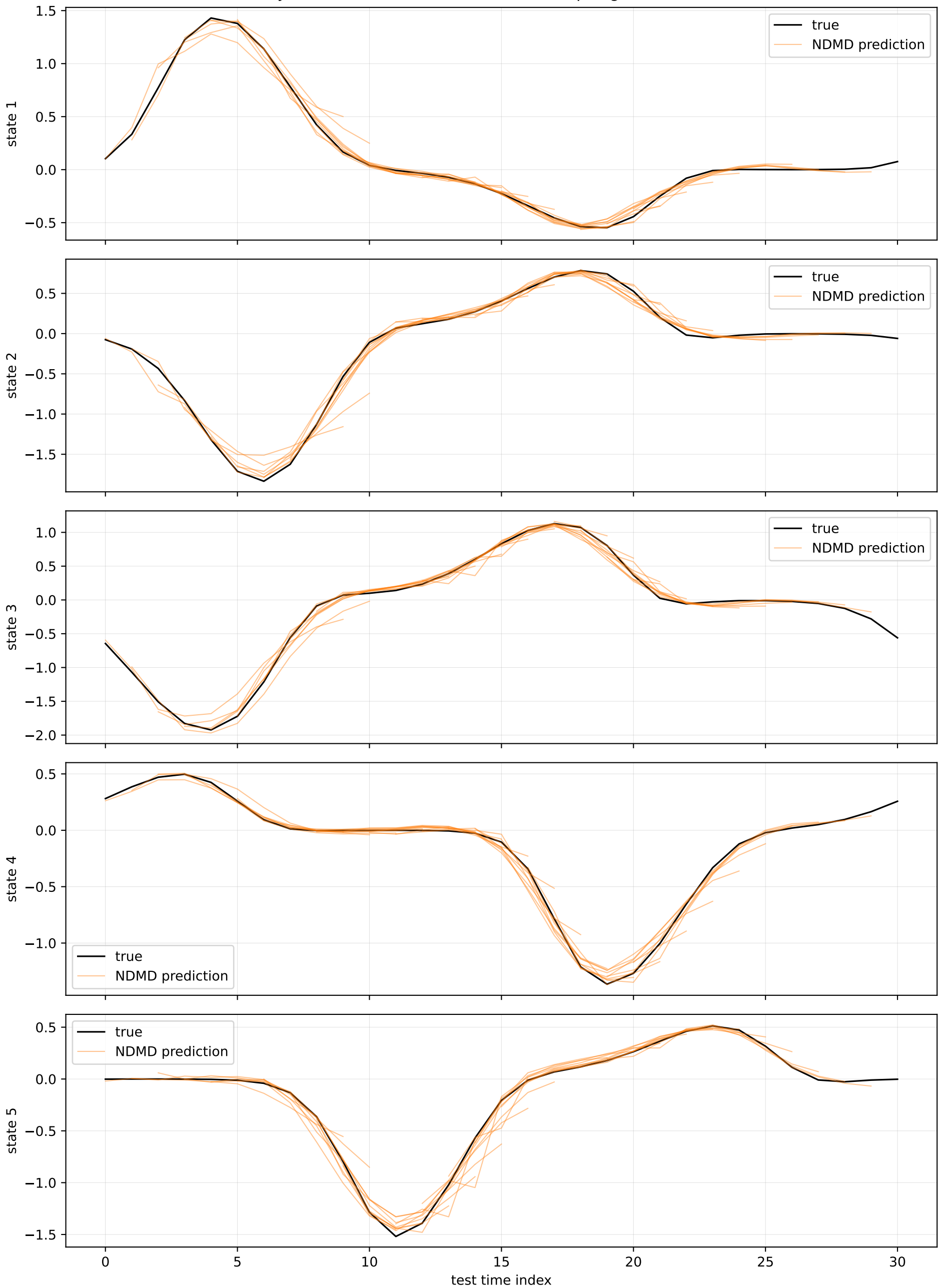
Cylinder Flow NDMD Prediction (10-step segments)
