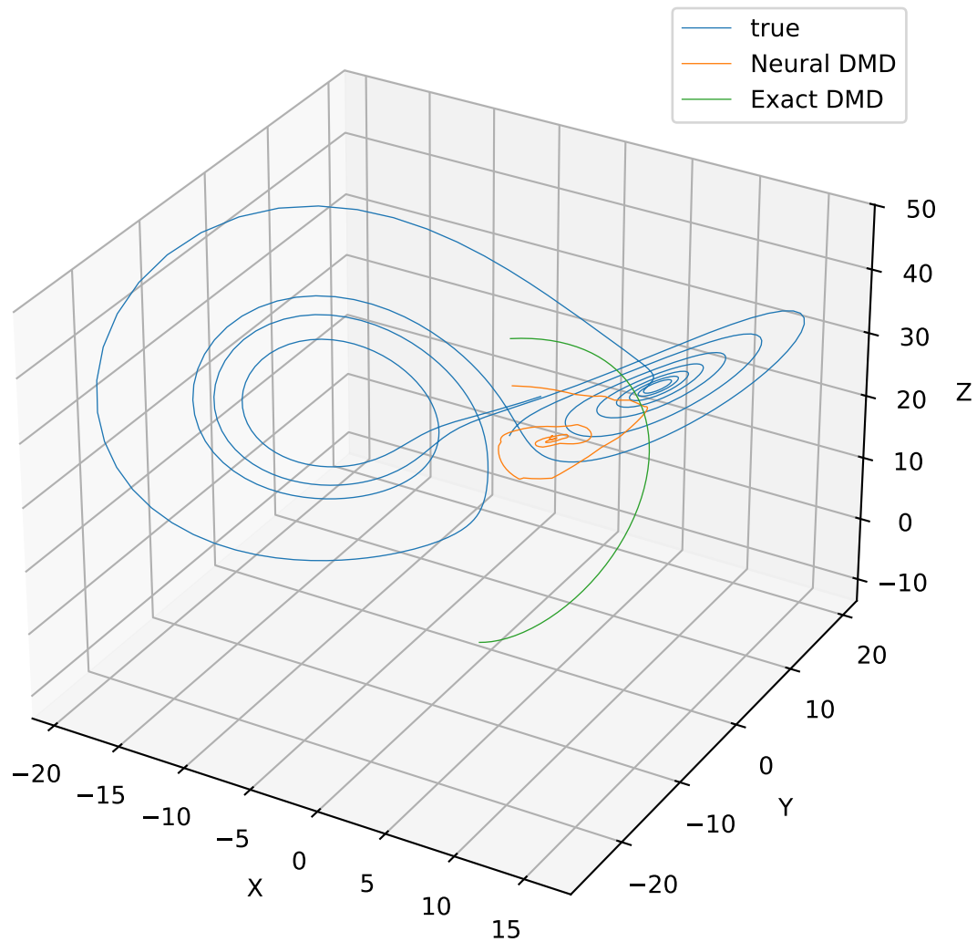
Lorenz Attractor Prediction Result
