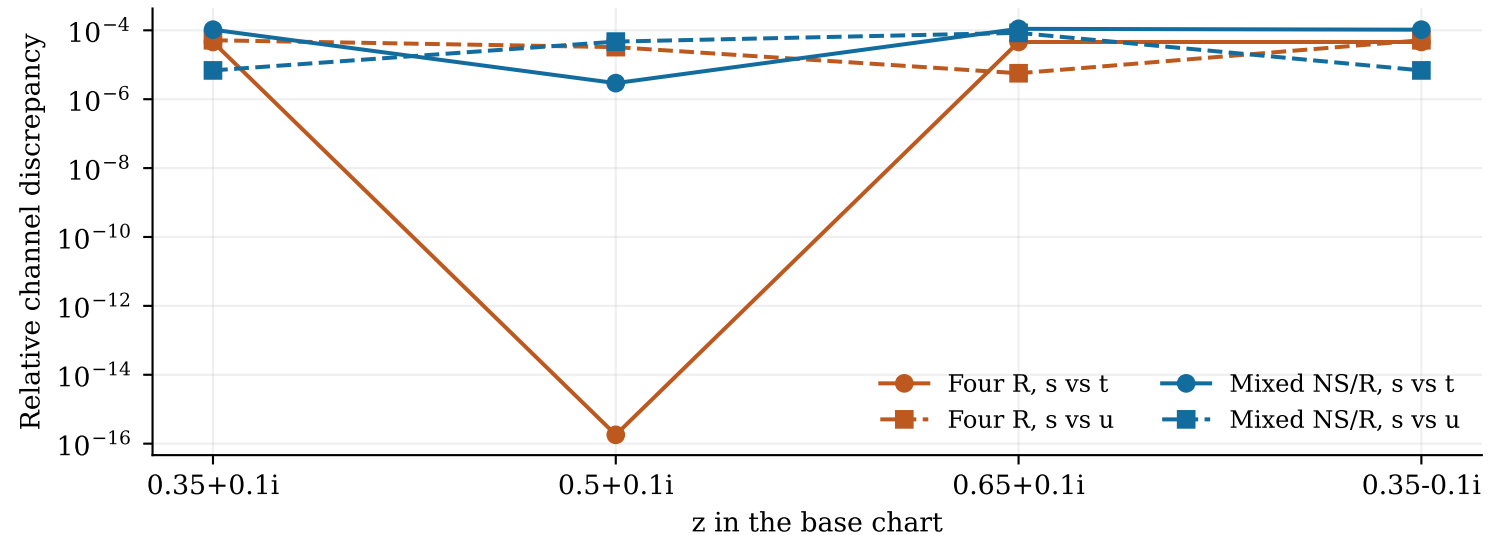
Fresh assembly of the order-5 production banks at \omega = i/4
