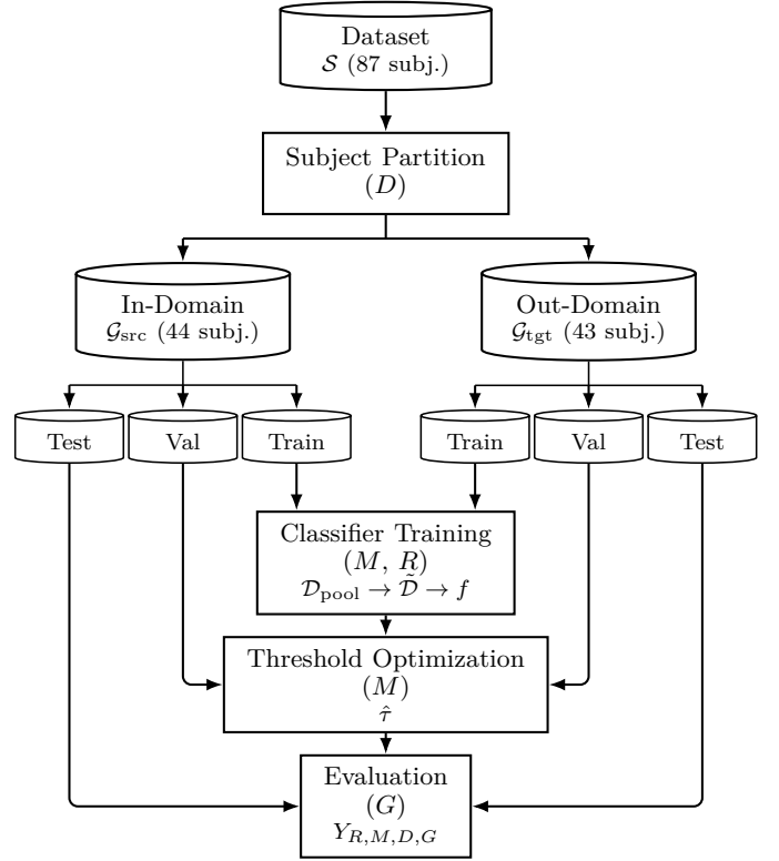
Fig. 3. Factorial experimental framework. Activity blocks are plain white: the upper half (Subject Partition \rightarrow In/Out groups \rightarrow per-subject 70/15/15 split) reuses the data-partition stage of the original combined-framework figure; the lower half mirrors the three terminal blocks of Fig. 1 (Classifier Training \rightarrow Threshold Optimization \rightarrow Evaluation), absorbing training-pool assembly, feature selection, rebalancing, hyperparameter tuning, and probability calibration into the Classifier Training block. Following the dependency chain D \rightarrow G \rightarrow M \rightarrow R , each factor is annotated inline at the activity it configures: Subject Partition by D (Distance Metric); Evaluation by G (Domain Membership); Classifier Training by M (Training Mode — selects the subject group whose Train splits form the training pool) and R (Rebalancing — applied to the training pool only, val/test pass through unchanged); Threshold Optimization by M as well, because the validation pool is drawn from the same M -dependent group (source for cross-domain, target for within-domain and mixed). Per-factor level sets are listed in Table I (Section IV-B); every (R, M, D, G) combination defines one factorial cell.
