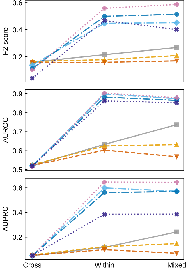
Fig. 6. Mode-dependent strategy performance across training modes. Line styles encode rebalancing families: solid = Baseline (grey), dashed = RUS (orange/vermillion for r=0.1/0.5 ), dash-dotted = SMOTE (light blue/blue for r=0.1/0.5 ), dotted = SW-SMOTE (pink/purple for r=0.1/0.5 ). Markers further distinguish strategies: square, up/down triangle, diamond, circle, plus, and cross. In Cross-domain, all strategies perform poorly; in Within/Mixed, SMOTE-based strategies sharply improve while RUS variants remain low—illustrating the R \times M interaction.
