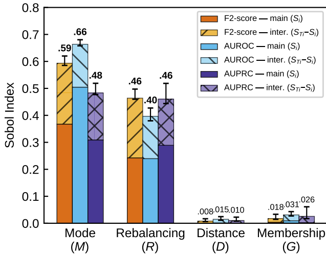
Fig. 5. Sobol sensitivity indices for the four factors. Solid bars: first-order indices ( S_i ); hatched bars: interaction contributions ( S_{T_i} - S_i ). Error bars: 95% bootstrap CIs on S_{T_i} . Mode and Rebalancing dominate; Distance and Membership are negligible.
