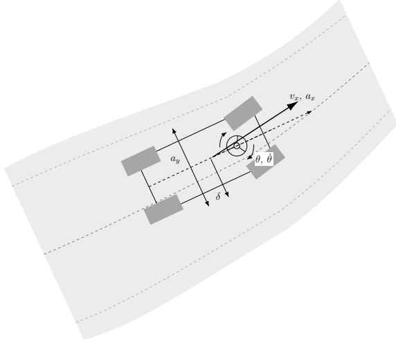
Fig. 2. Kinematic bicycle model coupling structure of the five vehicle-dynamics signals listed in Table II. Four of the five signals ( \delta , \dot{\delta} , a_y , e_{\text{lane}} ) are tied to the steering input \delta(t) through Eqs. (9)–(10); only longitudinal acceleration a_x is dynamically independent. Yaw angle \theta and yaw rate \dot{\theta} are shown for context but are not directly observed in this dataset.
