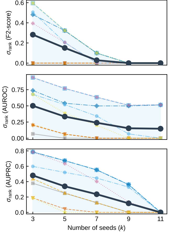
Fig. 7. Ranking stability ( \sigma_{\text{rank}} ) as a function of seed subset size k . Thick solid line with circles: mean \sigma_{\text{rank}} across all seven strategies; dashed line with squares and shaded band: maximum \sigma_{\text{rank}} . Thin lines show per-strategy convergence (line style encodes family): solid with square = Baseline; dashed with up/down triangles = RUS r=0.1/0.5 ; dash-dotted with diamond/circle = SMOTE r=0.1/0.5 ; dotted with plus/cross = SW-SMOTE r=0.1/0.5 . Monotonic convergence confirms that n = 12 seeds is sufficient.
