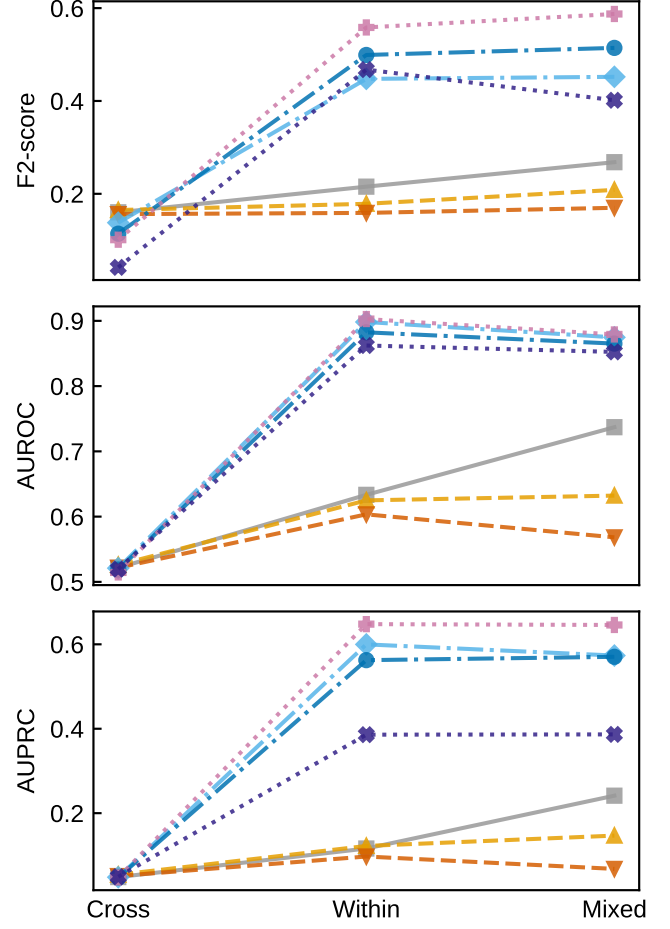
Fig. 5. Mode-dependent strategy performance across training modes. Line styles encode rebalancing families: solid = Baseline (grey), dashed = RUS (orange/vermillion for r=0.1/0.5 ), dash-dotted = SMOTE (light blue/blue for r=0.1/0.5 ), dotted = SW-SMOTE (pink/purple for r=0.1/0.5 ). Markers further distinguish strategies: square, up/down triangle, diamond, circle, plus, and cross. In Cross-domain, all strategies perform poorly; in Within/Mixed, SMOTE-based strategies sharply improve while RUS variants remain low—illustrating the R \times M interaction.
