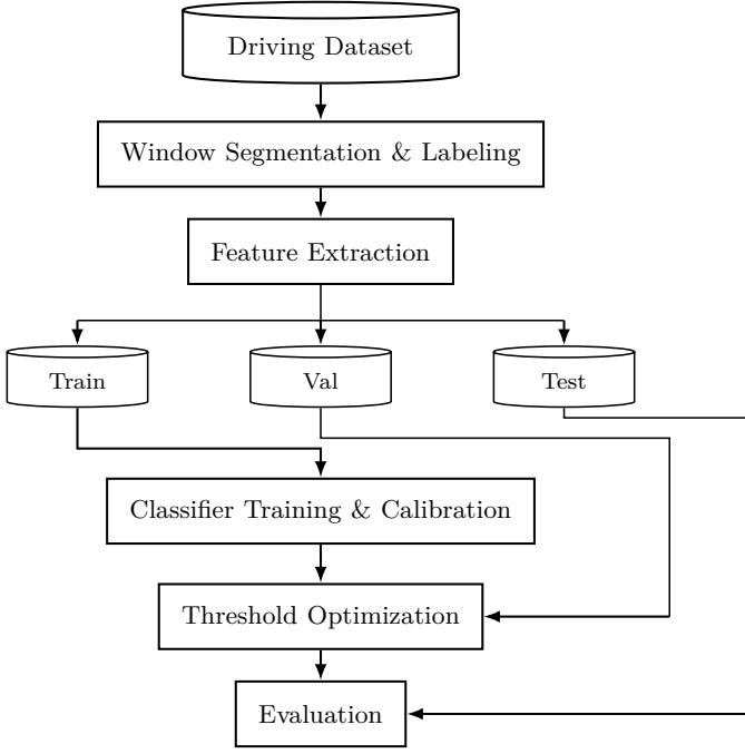
Fig. 1. Generic vehicle-dynamics-based DDD pipeline. Per-subject vehicle signals are segmented into labeled windows, features are extracted, and a chronological train/validation/test split is applied. The training set fits the classifier (which absorbs hyperparameter tuning and probability calibration as standard sub-steps); the validation set tunes the decision threshold; the test set is reserved for the final evaluation. This pipeline is shared, with minor variations, across most prior DDD studies; the four experimental factors specific to this work are introduced in Section IV (Fig. 2).
