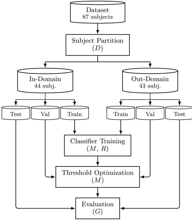
Fig. 2. Factorial experimental framework. Activity blocks are plain white: the upper half (Subject Partition \rightarrow In/Out groups \rightarrow per-subject 70/15/15 split) reuses the data-partition stage of the original combined-framework figure; the lower half mirrors the three terminal blocks of Fig. 1 (Classifier Training \rightarrow Threshold Optimization \rightarrow Evaluation), absorbing training-pool assembly, feature selection, rebalancing, hyperparameter tuning, and probability calibration into the Classifier Training block. Following the dependency chain D \rightarrow G \rightarrow M \rightarrow R , each factor is annotated inline at the activity it configures: Subject Partition by D (Distance Metric); Evaluation by G (Domain Membership); Classifier Training by M (Training Mode — selects the subject group whose Train splits form the training pool) and R (Rebalancing — applied to the training pool only, val/test pass through unchanged); Threshold Optimization by M as well, because the validation pool is drawn from the same M -dependent group (source for cross-domain, target for within-domain and mixed). Per-factor level sets are listed in Table I (Section IV-B); every (R, M, D, G) combination defines one factorial cell.
