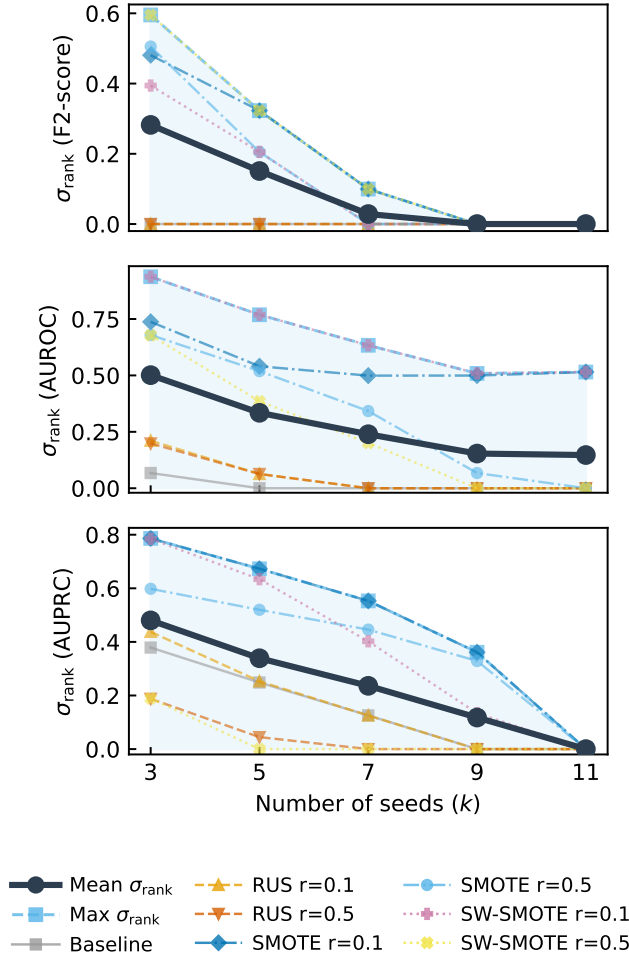
Fig. 6. Ranking stability ( \sigma_{\text{rank}} ) as a function of seed subset size k (rows: F2-score, AUROC, AUPRC). Thick line: mean \sigma_{\text{rank}} across the seven strategies; dashed line with shaded band: maximum \sigma_{\text{rank}} . Thin lines show per-strategy convergence (see legend). Monotonic convergence confirms that n = 12 seeds is sufficient.
