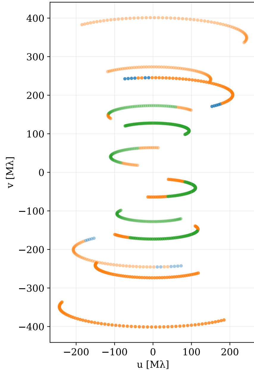
Short baselines ( r \leq 1 \text{ G}\lambda )
