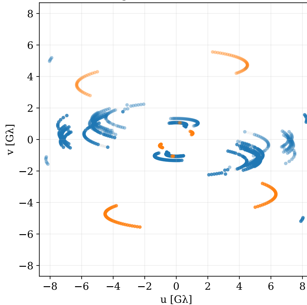
Long baselines ( r > 1 \text{ G}\lambda )
