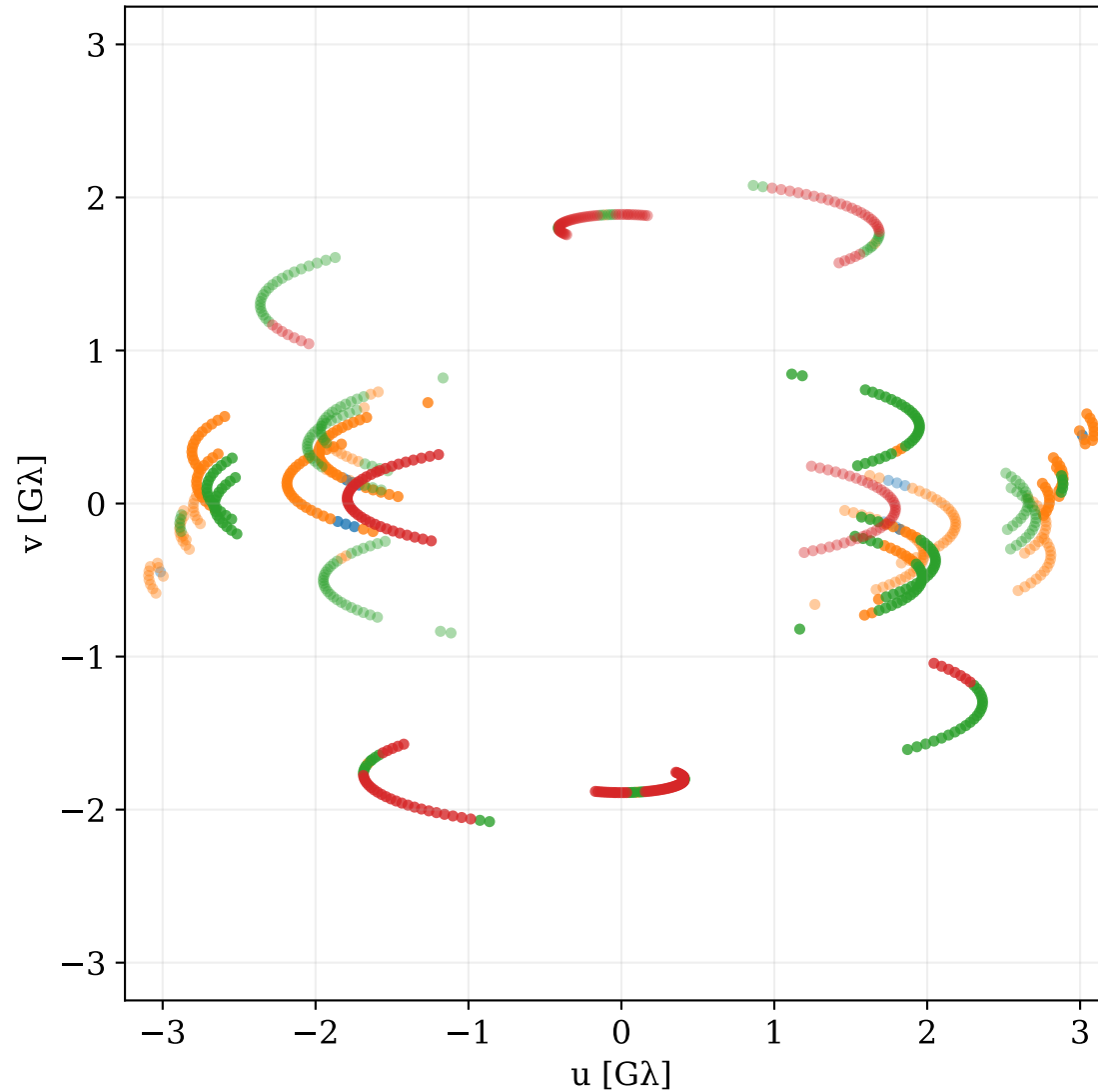
Long baselines ( r > 1 \text{ G}\lambda )
