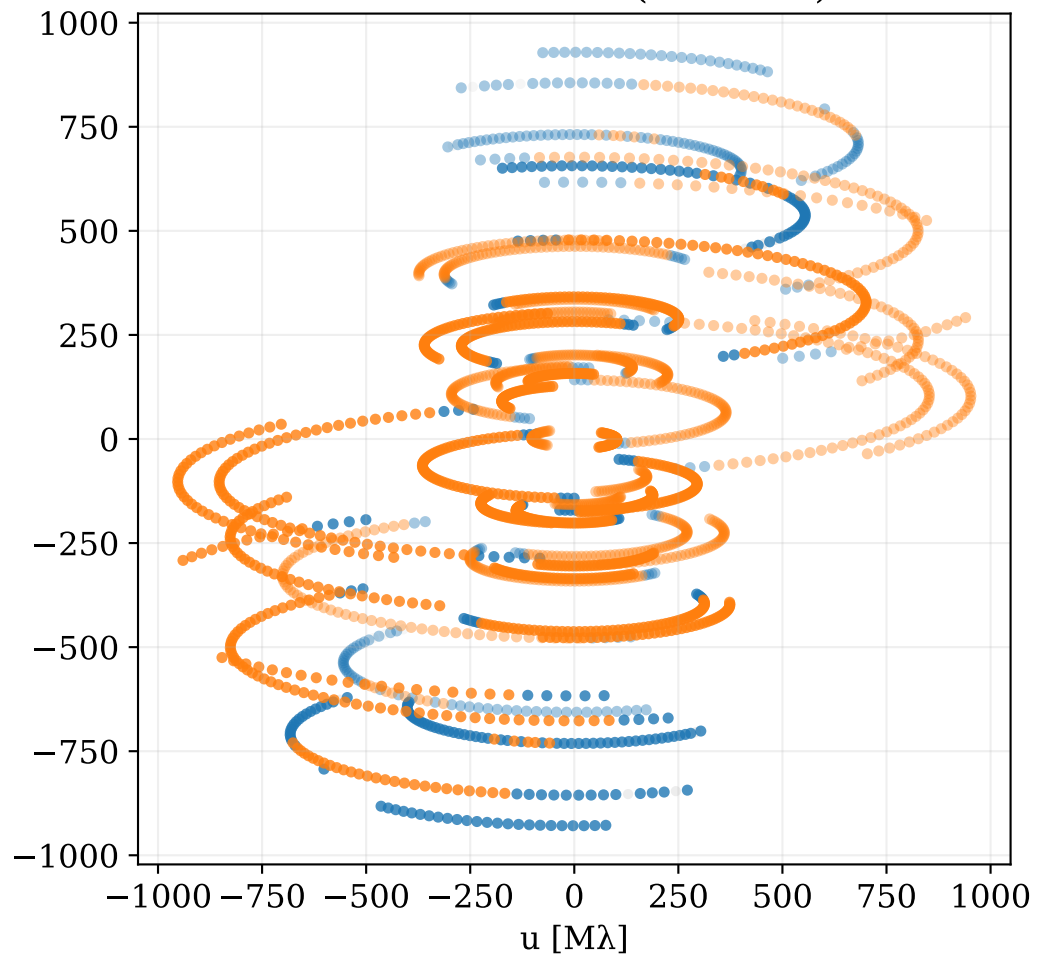
Short baselines ( r \leq 1 \text{ G}\lambda )
