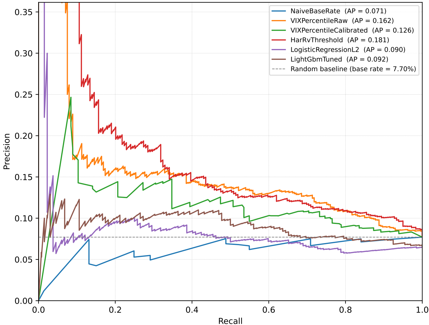
Precision-recall curves (h=10, d=5%)
