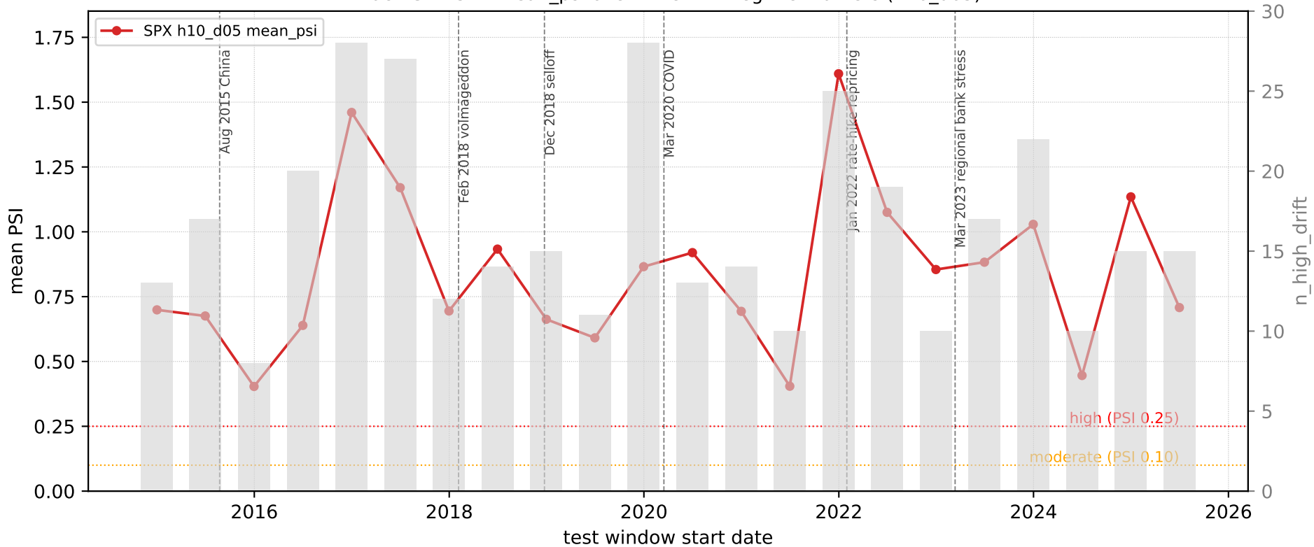
Track G — SPX mean_psi over time with regime markers (h10_d05)
