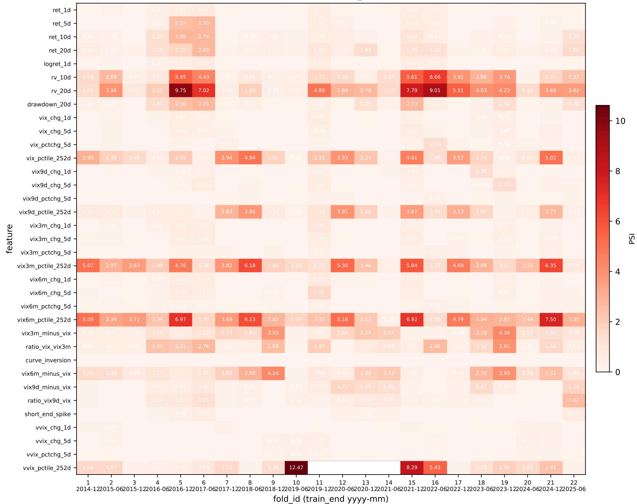
Track G — SPX per-feature PSI by fold (h10_d05); cells &gt; 0.25 annotated
