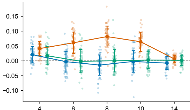
Weighted UniFrac — dilution tier (scale 0.5)
