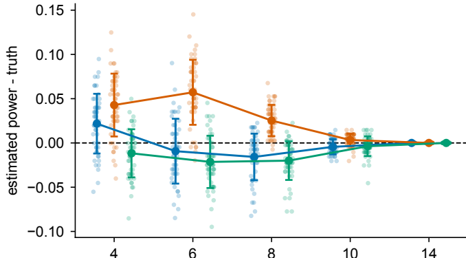
Bray-Curtis — baseline tier (scale 1.0)
