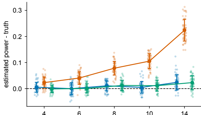
Bray-Curtis — dilution tier (scale 0.5)
