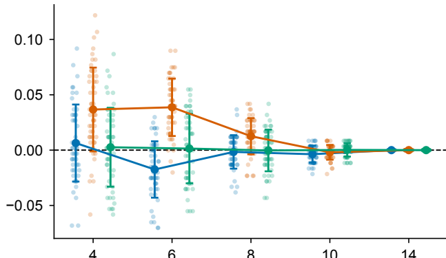
Weighted UniFrac — baseline tier (scale 1.0)
