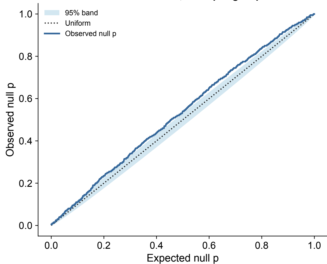
Null calibration, n=14 per group
