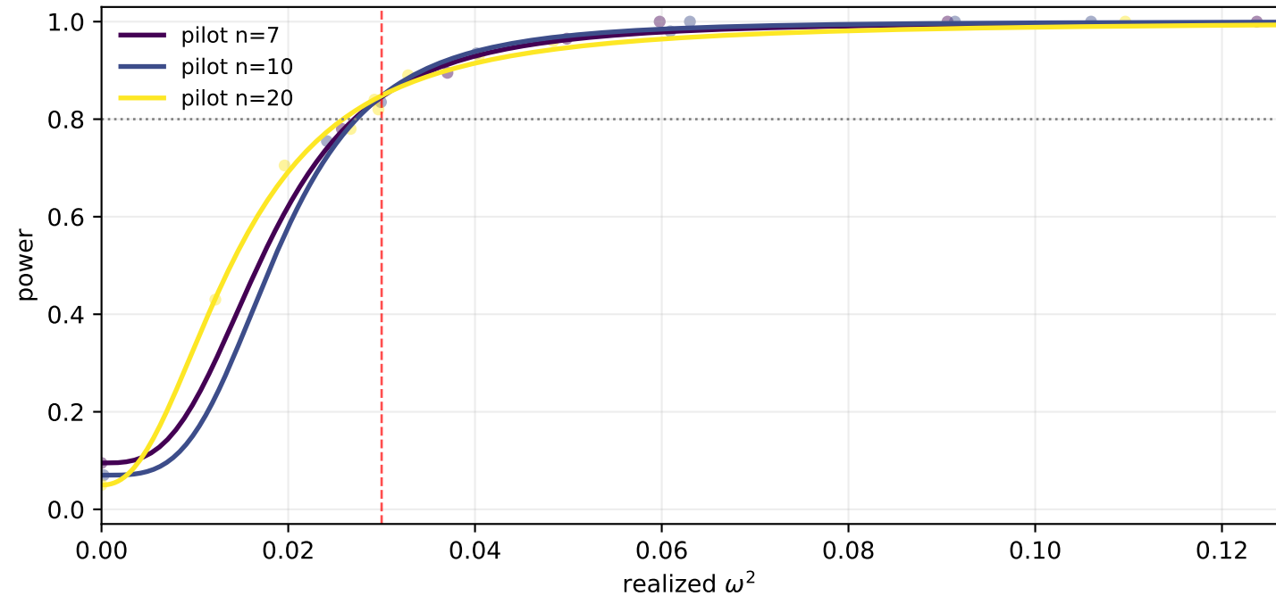
Gene pilot extrapolation (eval n=80)
