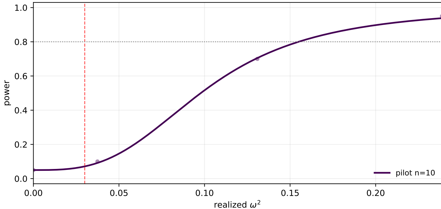
Gene pilot consistency (eval n=10)
