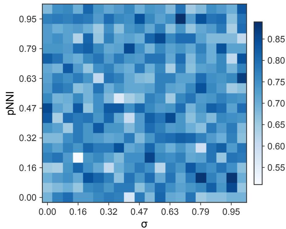
Metaproteomics — Baseline Power (PhyloFunc, 7 vs 7)
