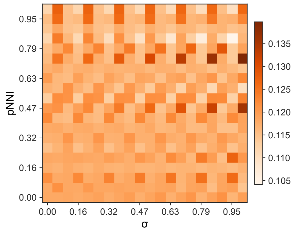
Metaproteomics — Baseline \omega^2 (PhyloFunc, 7 vs 7)
