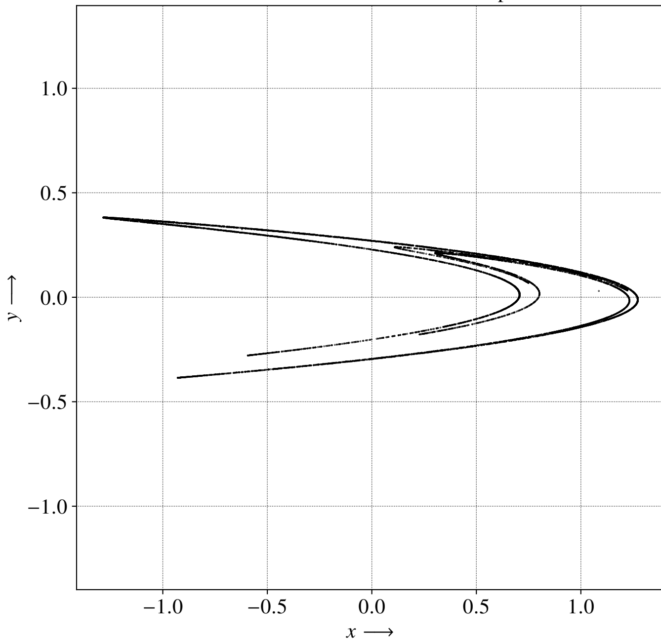
Phase Portrait of the Hénon Map
