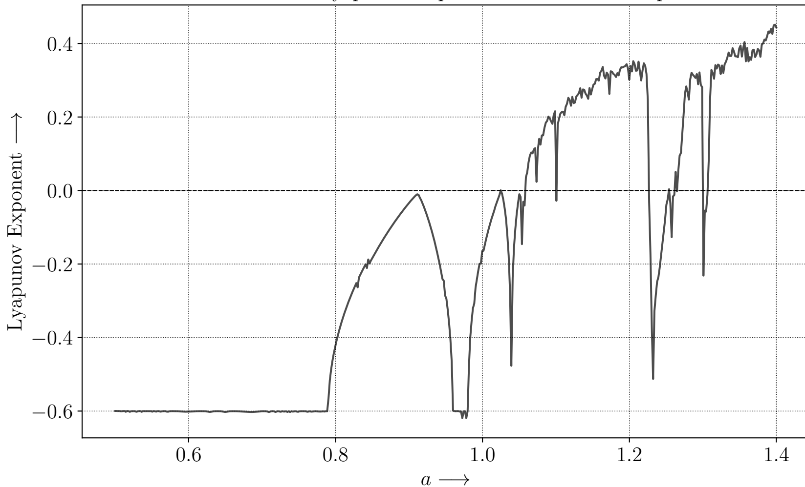
Maximum Lyapunov Exponent of the Henon Map
