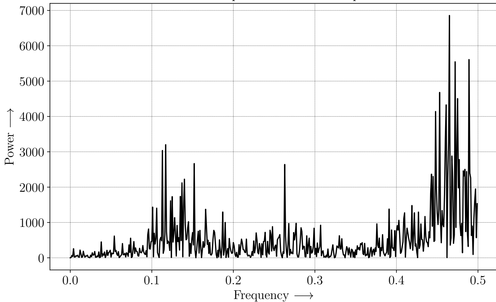
Power Spectrum of Henon Map
