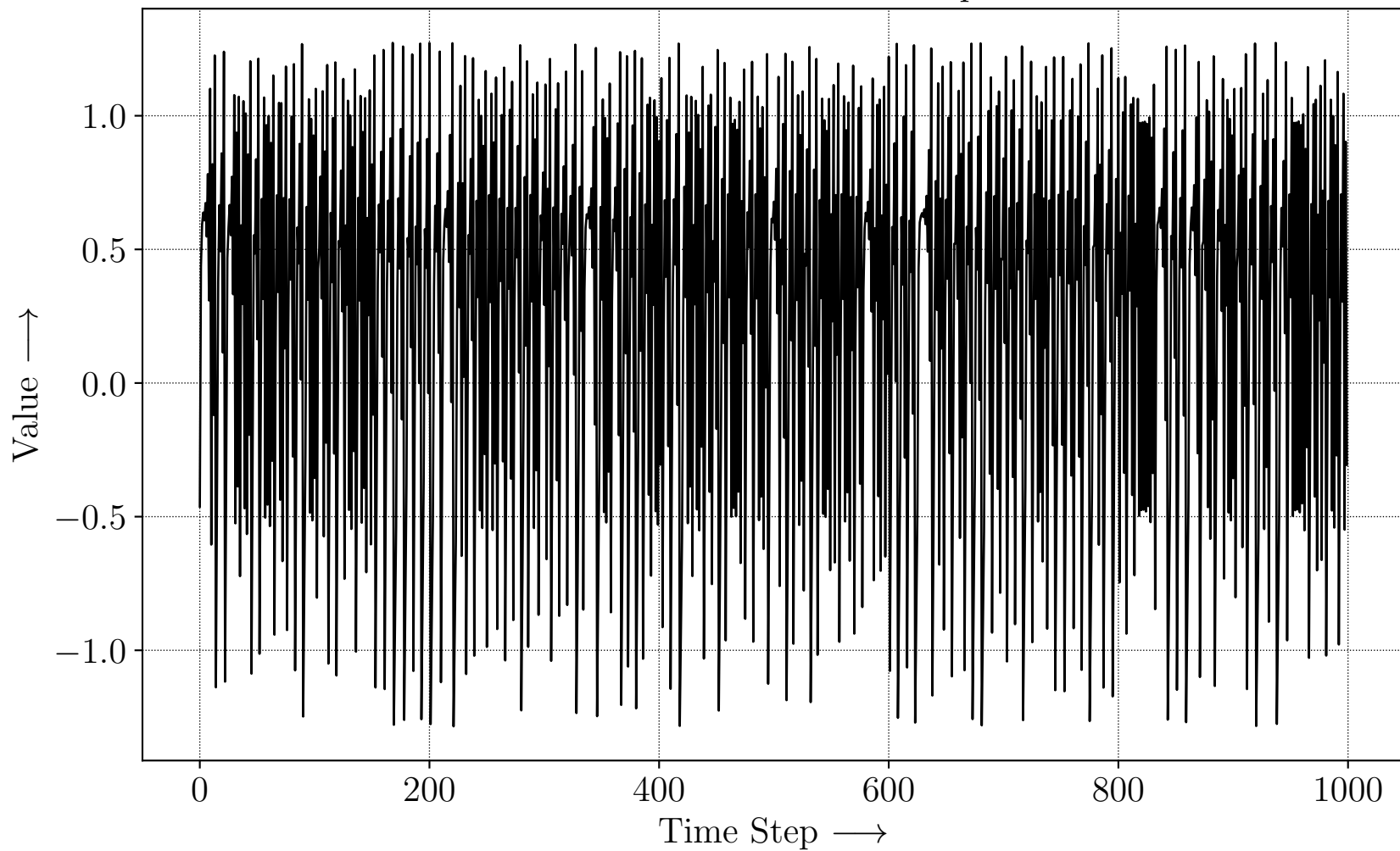
Time Series of Henon Map
