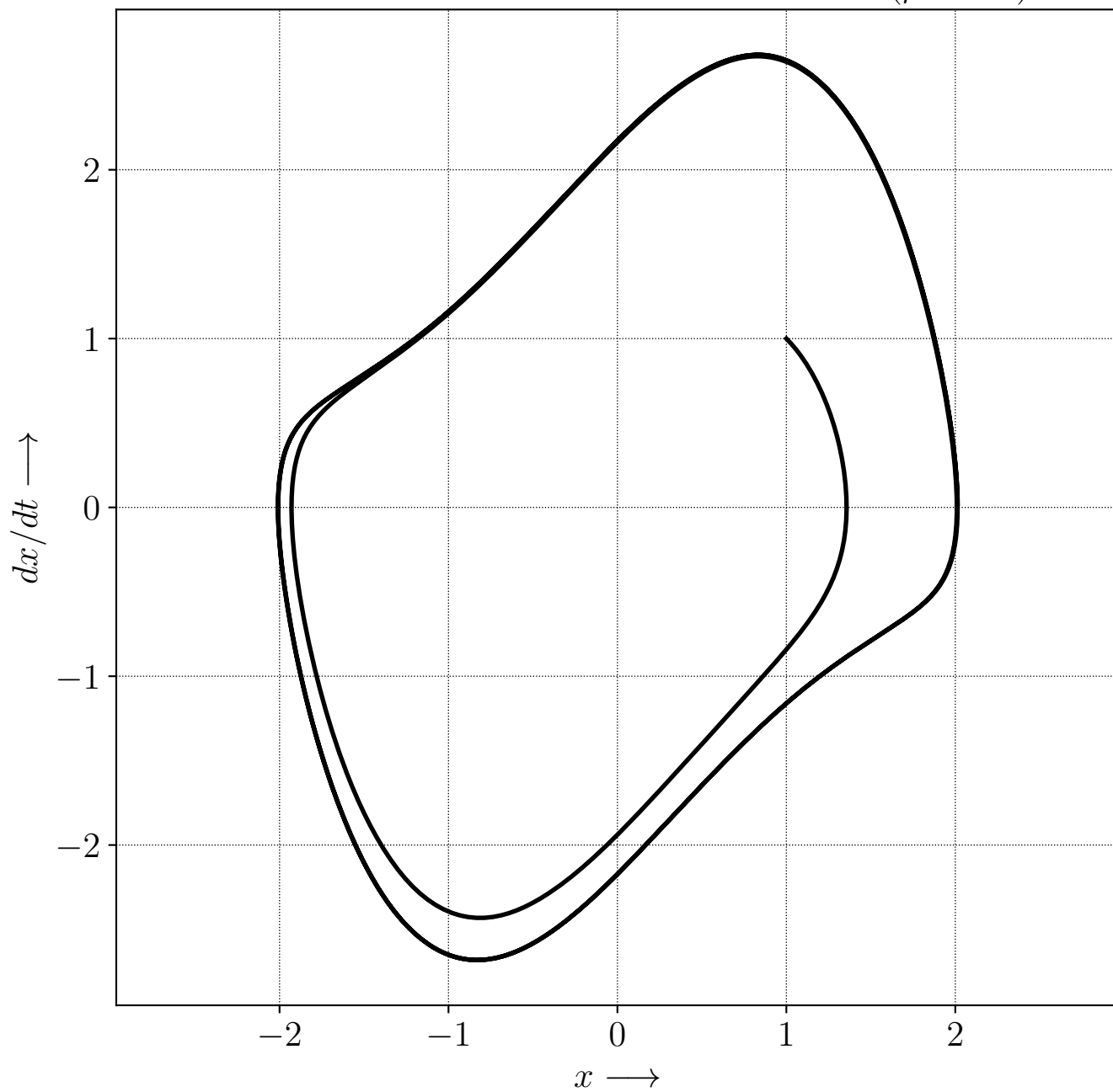
Phase Portrait of the van der Pol Oscillator ( \mu = 1.0 )
