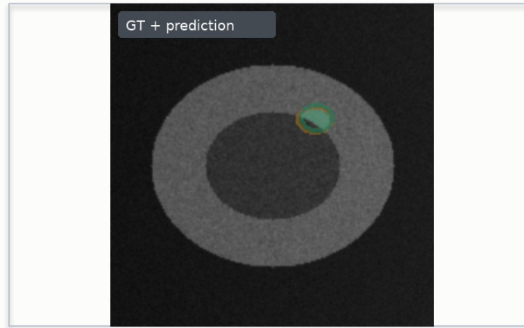
GT / prediction
