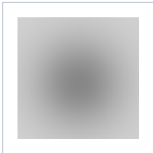
Synthetic image
