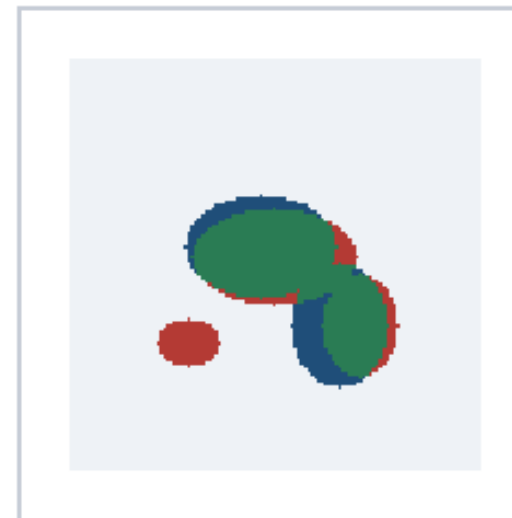
FP/FN overlay
