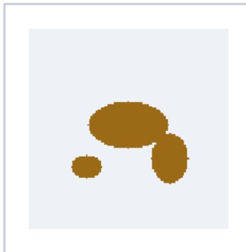
Prediction
