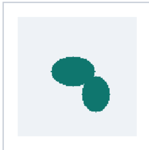
GT mask
