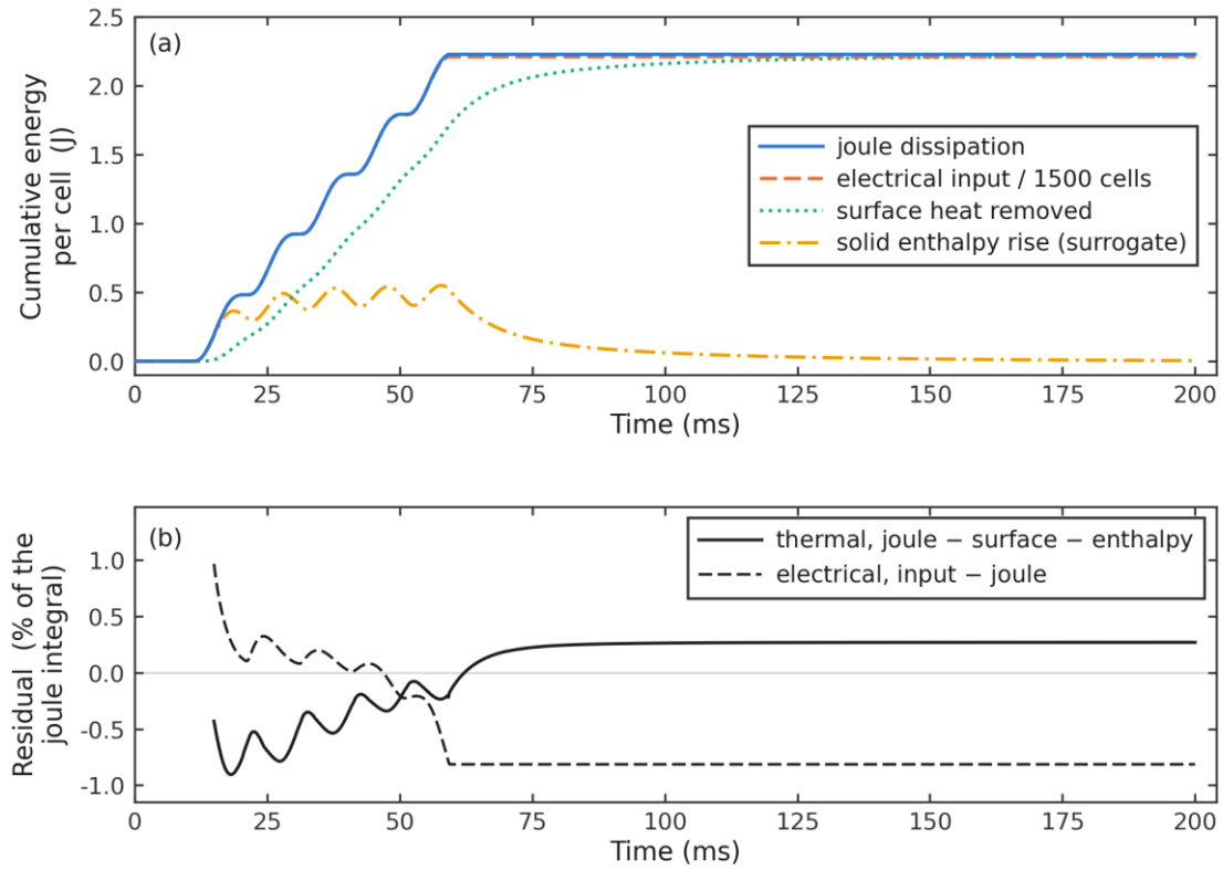
Figure 4.11 Energy balance of the base case.
