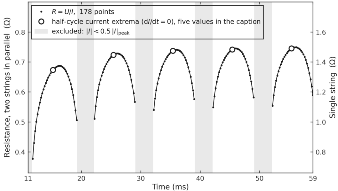
Figure 4.8 Device equivalent resistance during the fault.
