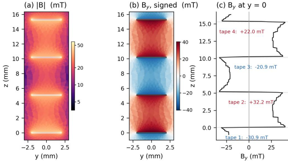
Figure 4.16 Cross-section flux density at the fault peak (15.2 ms, 50 ms clearing case).
