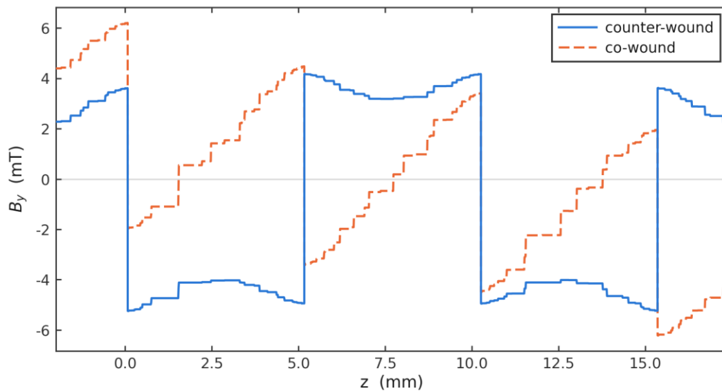
Figure 4.18 B_y through the four-tape stack, counter-wound against co-wound (rated operation).
