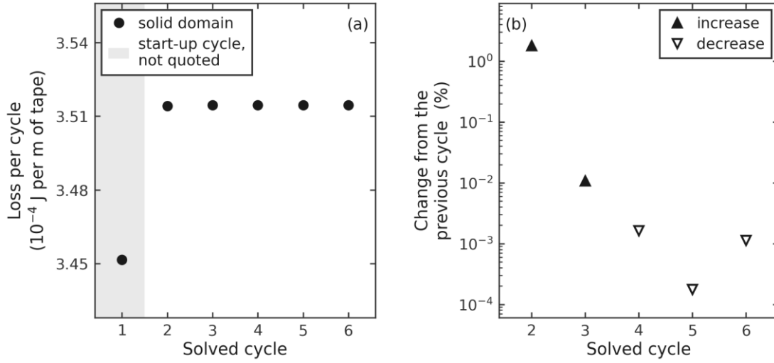
Figure 4.15 Cycle-by-cycle AC loss and inter-cycle drift at rated operation.
