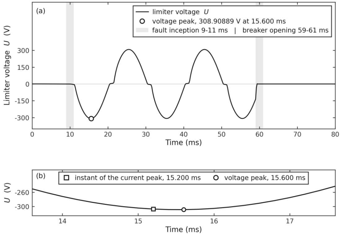
Figure 4.3 SFCL terminal voltage with a close-up of the first peak.
