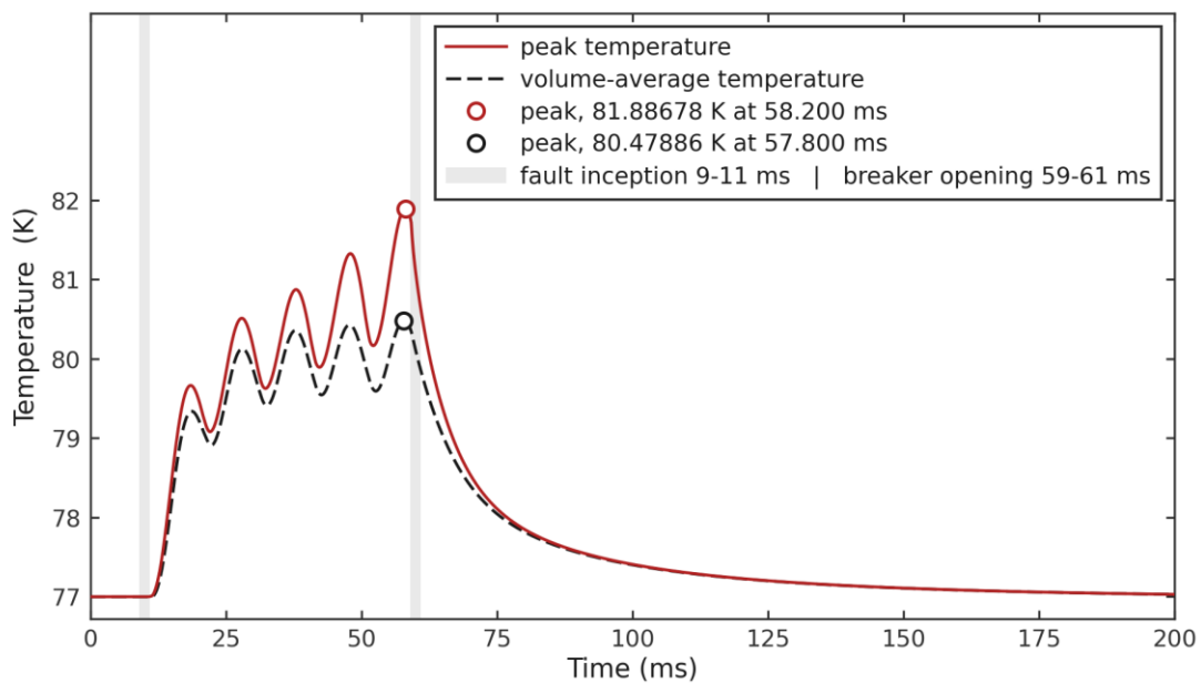
Figure 4.4 Volume-average and superconducting-layer extremum temperature, base case.
