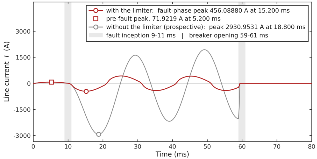
Figure 4.1 Line current with and without the SFCL.
