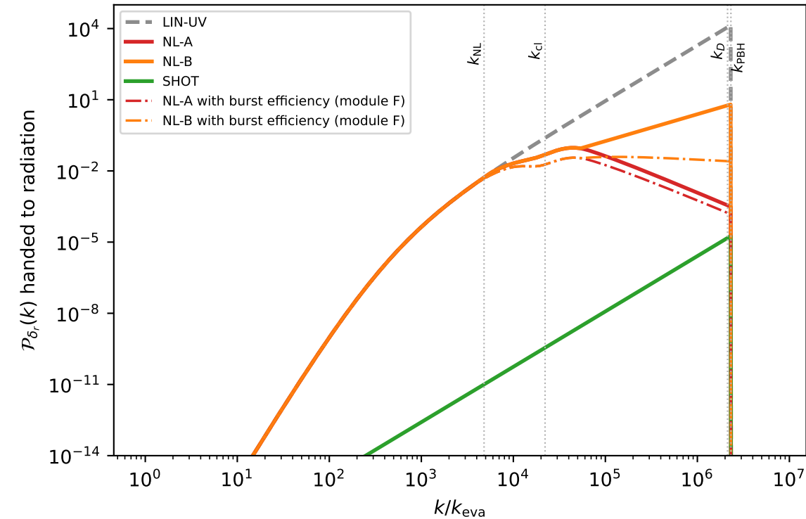
monochromatic: 10^4 g , \beta_f = 10^{-6}
